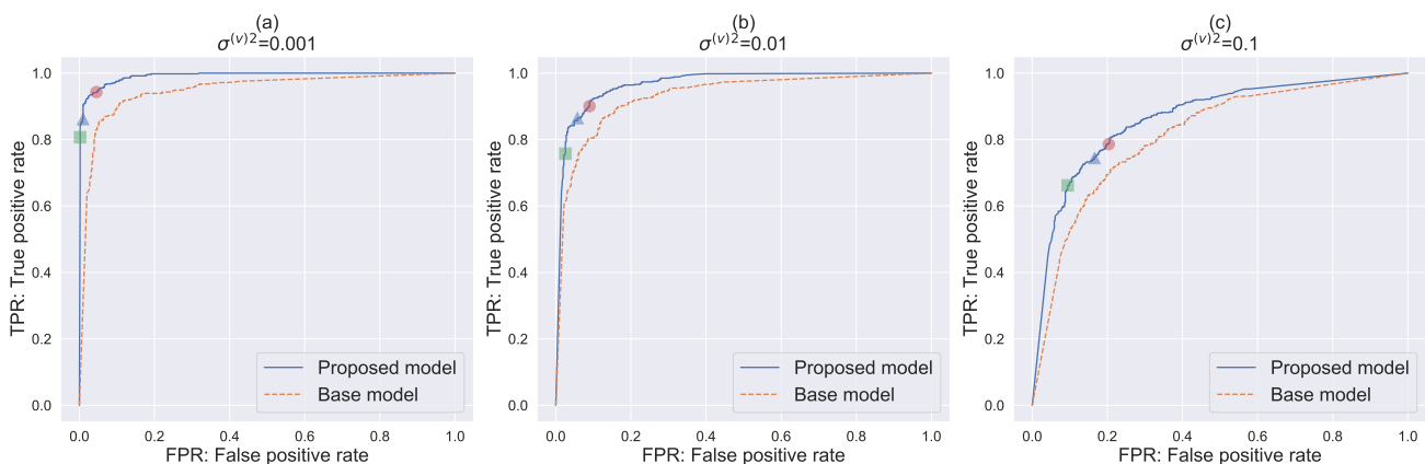
Figure 3: The AUC-ROC curve for identifying responders based on the estimated posterior distributions of \eta in the synthetic datasets of N = 85 and (d_1, d_2, d_3, d_4) = (29, 43, 71, 85) using the proposed model ( \mu_{\max} = \nu_{\max} = 5 ) and the base model ( \mu_{\max} = \nu_{\max} = 0 ). The x - and y -axes indicate the false positive and true positive rates, respectively. The blue and orange dashed lines indicate the results for \mu_{\max} = \nu_{\max} = 5 and \mu_{\max} = \nu_{\max} = 0 , respectively. The red circle, blue triangle, and green square indicate the performance of responder identification with the threshold of the probability of \eta > 0.5, 0.7 , and 0.95 , respectively, when \mu_{\max} = \nu_{\max} = 5 .
