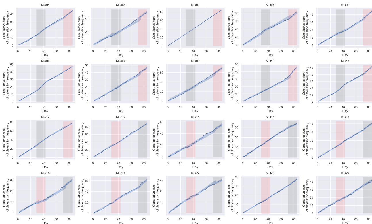
Figure 7: Data used and predictive distributions. The x - and y -axes indicate the day and cumulative sum of the defecation frequencies, respectively. The blue line and the blue area indicate real data and the 2.5% and 97.5% percentiles of predictive distributions, respectively. The red and black areas indicate the intake periods of the target probiotic and placebo, respectively.
