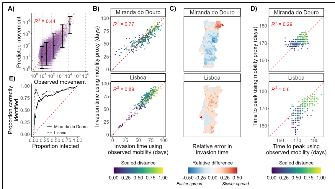
Figure 3: Mobility predictions and epidemic simulations for Portugal. A) Predicted numbers moving between Portuguese ADM2 units vs observed numbers from mobile phone call records. Each purple dot represents a pair of ADM2 units. The black dots show the median predicted value (y value) versus the median observed value in each bin (where the bins are marked with grey dashed lines). Error bars show the 2.5% and 97.5% quantiles of the predicted values in that bin. B) and D) show respectively the median invasion time ( t_i^{first} ) and the median peak time ( t_i^{peak} ) amongst residents of each spatial unit (represented by a dot) across all simulations where an epidemic was successfully seeded. Plots compare the times when using observed mobility patterns (x-axis) vs the mobility proxy (y-axis) from our central scenario in the epidemic model (see Methods). The colour represents the normalised distance of each patch from the seed location (shown by the title of each grid), calculated by dividing the distance from the seed by the maximum distance from that seed. The red dashed line is where y = x . C) Maps of the relative error in invasion time in each spatial unit when using the mobility proxy vs observed data. Blue shading indicates the invasion time occurred earlier when using the mobility proxy, while red shading indicates a later invasion time when using mobility proxies. We use a relative scale, calculated as the difference between invasion time using mobility proxy and in the baseline (using the empirical mobility data), divided by the largest invasion times across all locations when using the proxy. The seeding location is marked with a red triangle. E) Invasion order similarity ( p_n^{first} ). The y-axis shows the proportion of the first n patches invaded in an epidemic model using observed mobility that were also among the first n locations invaded when a mobility proxy was used in the epidemic model. n is the proportion shown on the x-axis. The two lines show different seed locations. The dashed red line shows the expected value if locations are chosen randomly.
