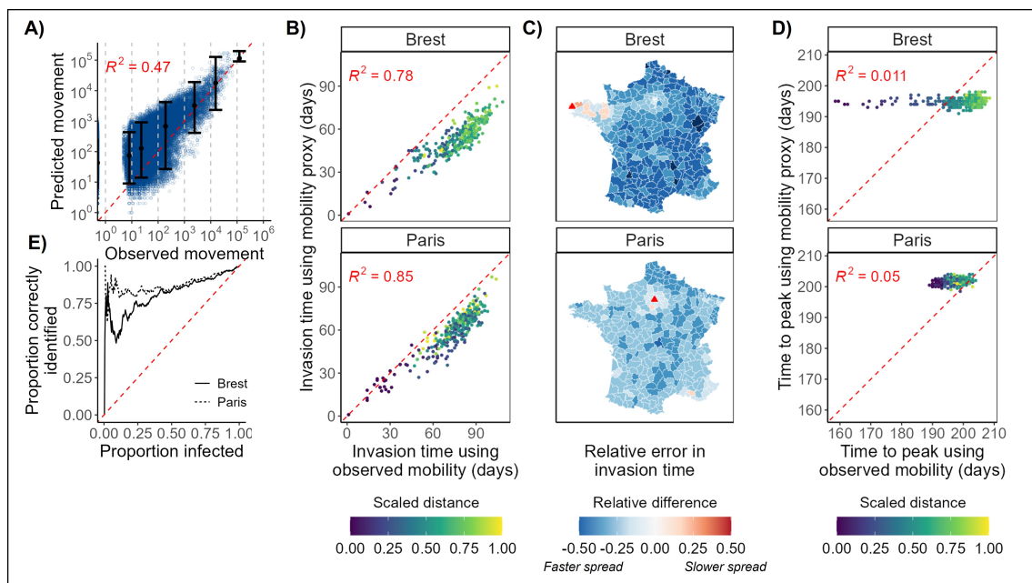
Figure 4: Mobility predictions and epidemic simulations for France. Figure details as in Fig. 4 except here A) shows predicted numbers moving between French ADM3 units vs observed numbers from mobile phone call records. Each blue dot represents a pair of ADM3 units.
