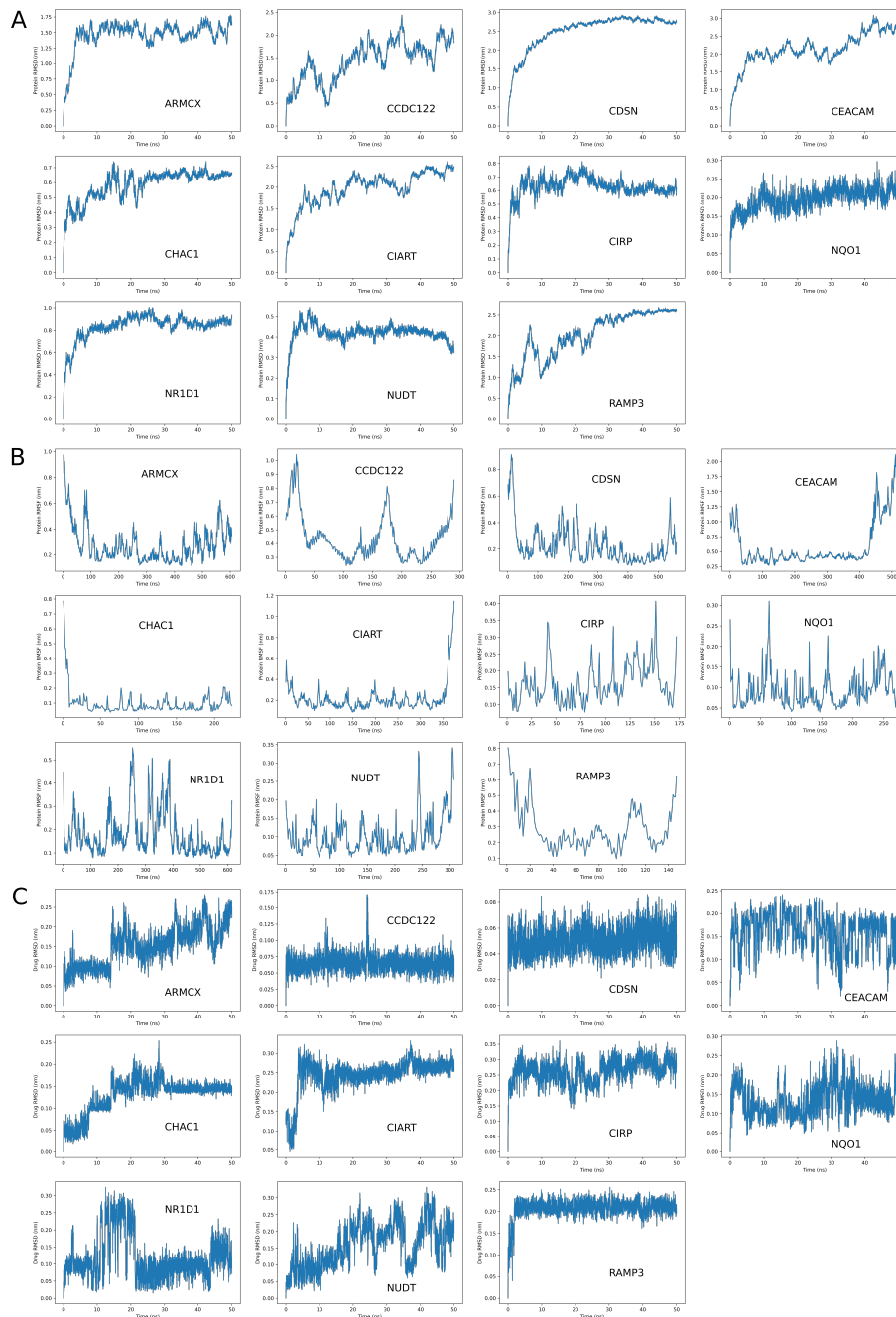
71 Figure 6. The RMSD and RMSF of MD simulation. A. The RMSD of proteins. B. The 72 RMSF of proteins. C. The RMSD of each molecular of proteins.
