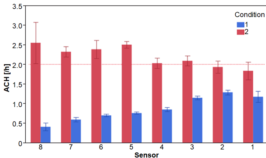
248 Figure 4. Estimated compartmental air change per hour (ACH) according to sensor. 249 Error bars indicate a 95% confidence interval.
