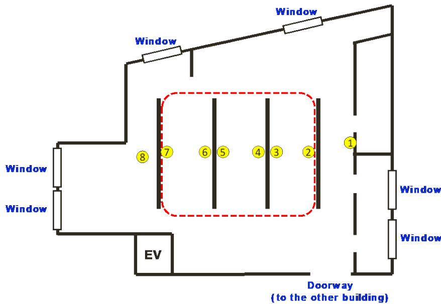
148 Figure 1. Layout of workplace and location of CO 2 sensors.
