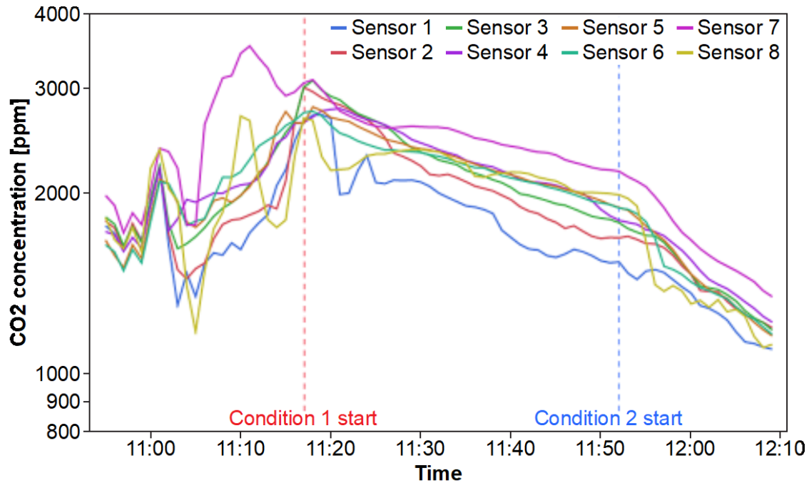
209 Figure 2. CO 2 concentration observed during experiments.
