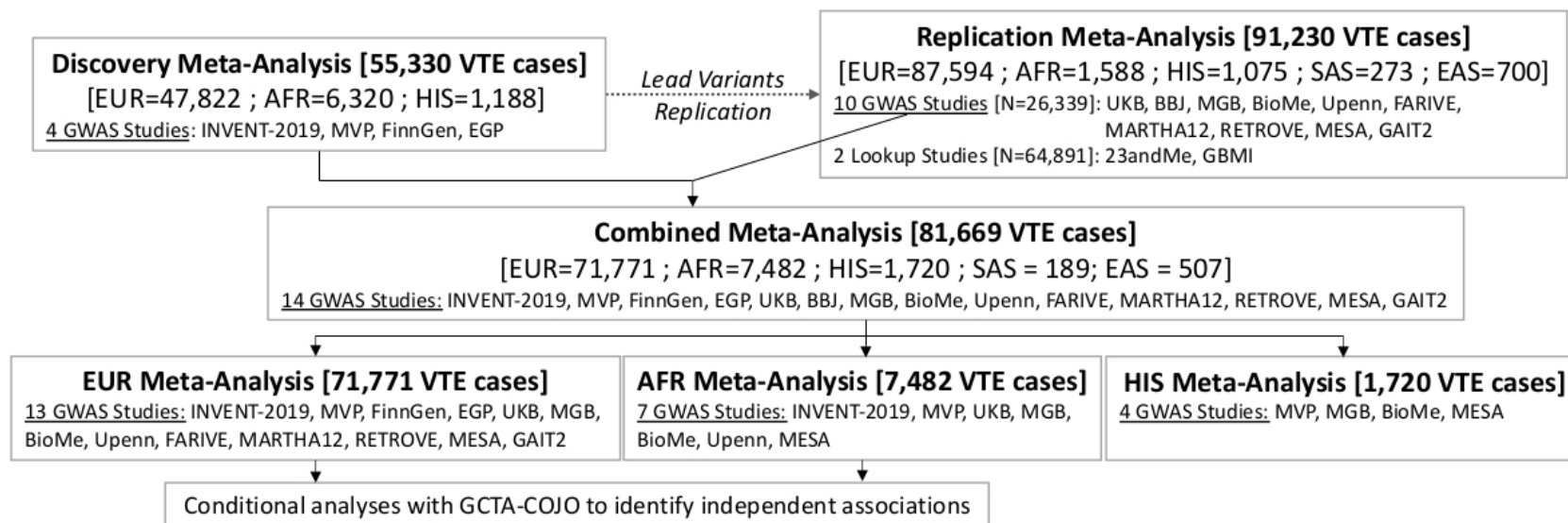
Figure 1: Analyses Workflow
