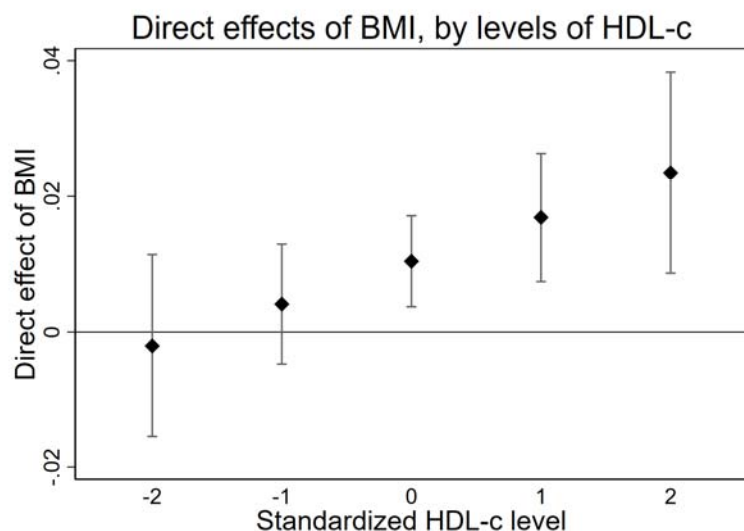
Figure 2: Excess relative risk of dementia due to direct effects of BMI, with HDL-c levels fixed at -2 to 2 standard deviations from the mean. Estimates were obtained from a mediation model with BMI as exposure, HDL-c as the mediator, and dementia as the outcome, with 4-way decomposition into direct effects, reference interaction, mediated interaction, and pure indirect effects. A linear regression model was used for the effect of BMI on HDL-c, and an accelerated failure time for the joint and interactive effects of BMI and HDL-c on time to dementia. The model was adjusted for age, sex, education, and study.
