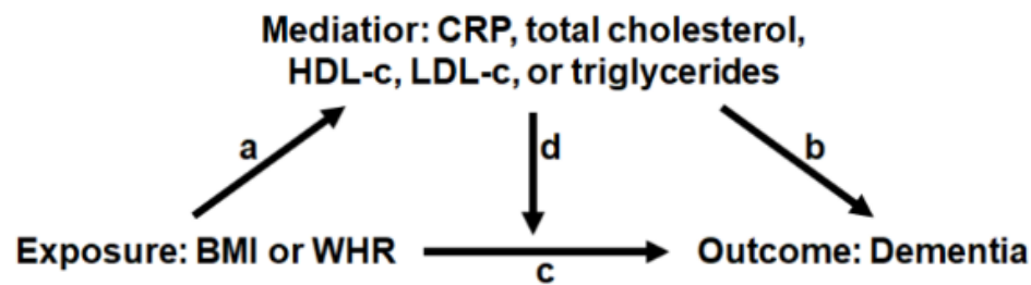
Figure 1: Directed acyclic graph for the relationship between adiposity and dementia, and mediation through CRP or lipid levels. Mediation effects are decomposed into controlled direct effects (through arrow c.), reference interaction (through arrows c. and d.), mediated interaction (through arrows a., c., and d.), and pure indirect effects (through arrows a. and b.).
