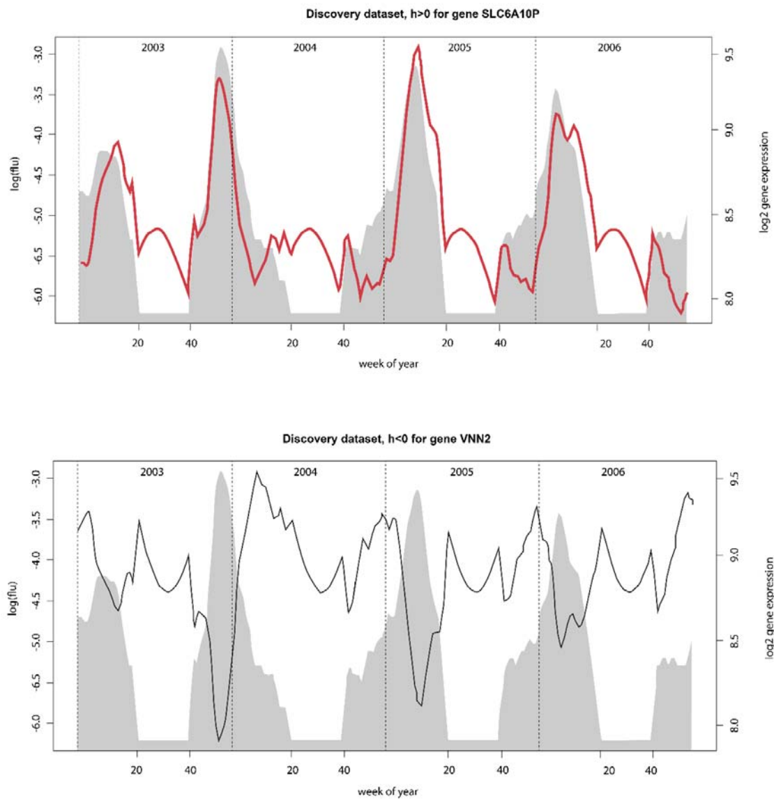
Figure 7. Gene expression trajectories for gene SLCA6A10P (largest h_g > 0 , upper panel, red line) and gene VNN2 (largest h_g < 0 , lower panel, black line) in relation to the estimated smoothed log flu intensities (grey shaded) 2003-2006
