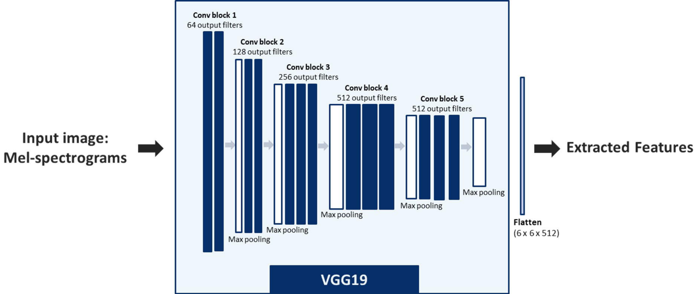
Figure 2. VGG19 Feature extraction
