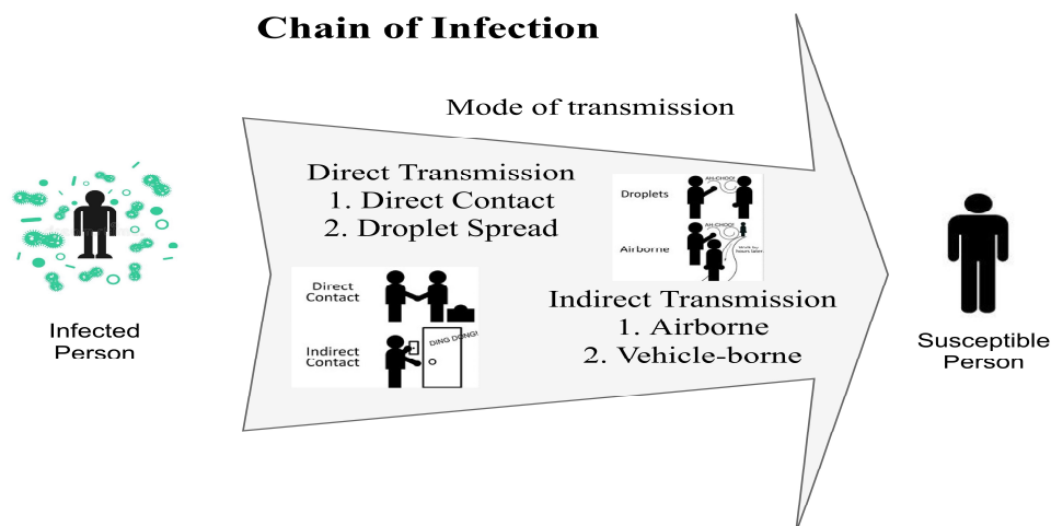
Figure 3: Chain of Infection
