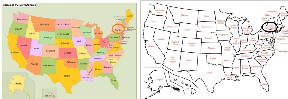
Figure 2: Population wise comparison of Indian places with USA states
