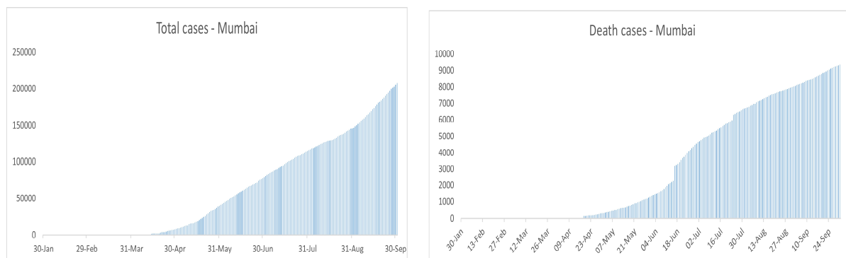
Figure 10: (a) Day-wise total cases of Mumbai, (b) Day-wise total death of Mumbai
