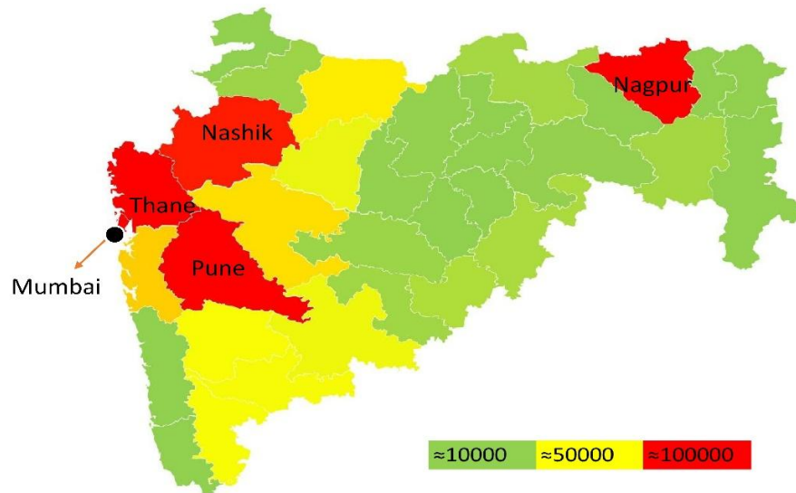
Figure 1: Geographically COVID-19 case distribution in the state of Maharashtra
