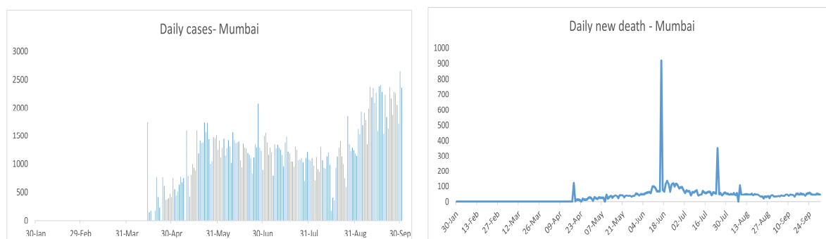
Figure 11: (a) Daily new cases of Mumbai, (b) Daily new death cases of Mumbai
