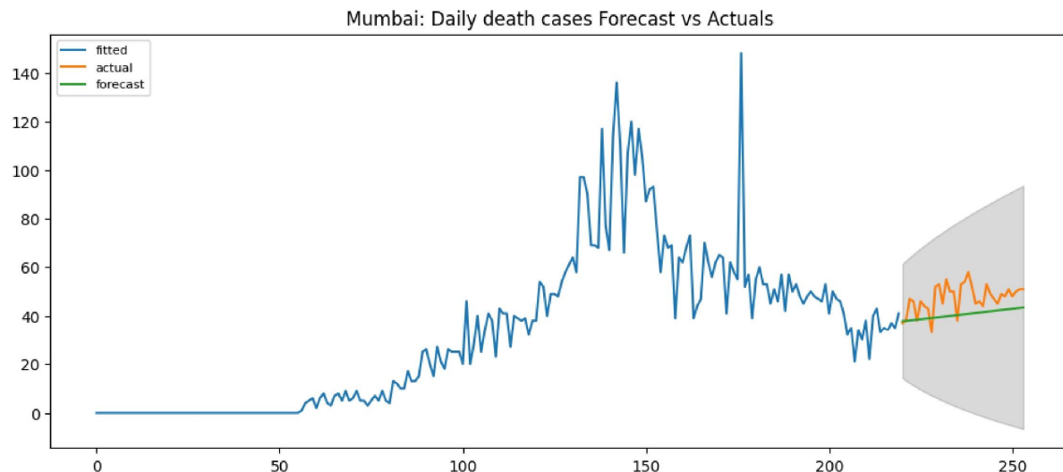
Figure 16: Compare actual and forecast data for daily death cases with an interval of 95%
