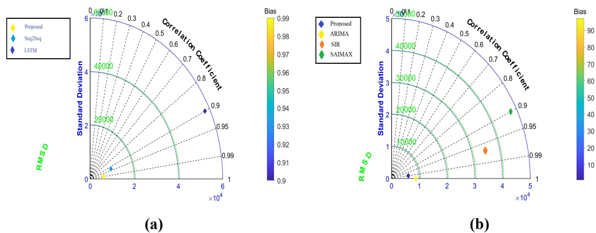
Figure 17: (a) Taylor diagram and proposed method compare with the deep learning prediction models, (b) Taylor diagram of proposed method compare with the state-of-the-art methods
