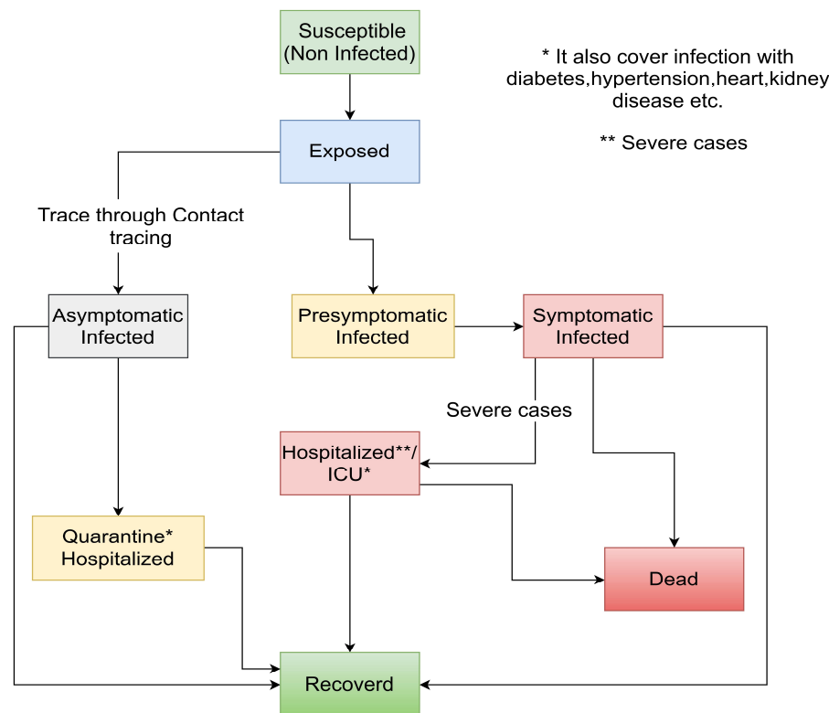
Figure 6: Flow of proposed model
