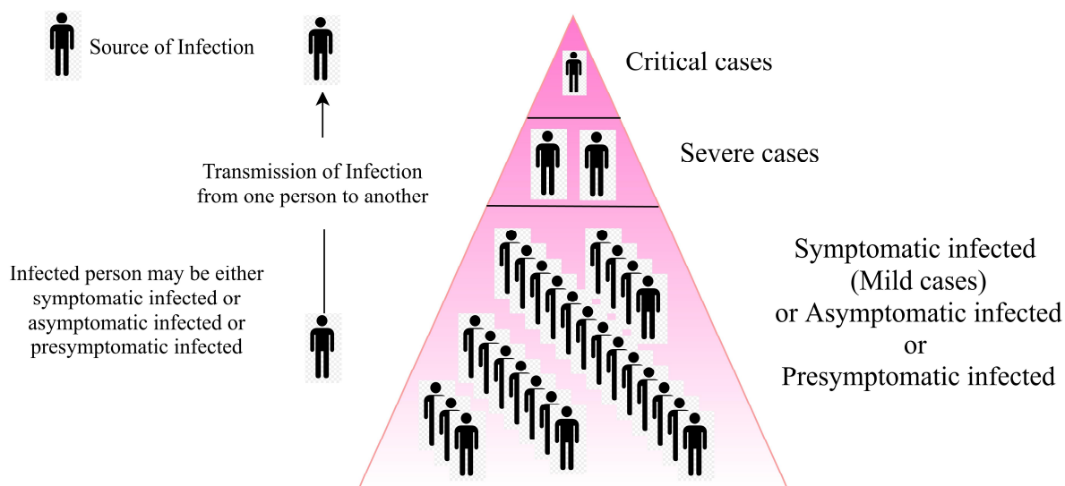
Figure 4: Hierarchy of infection
