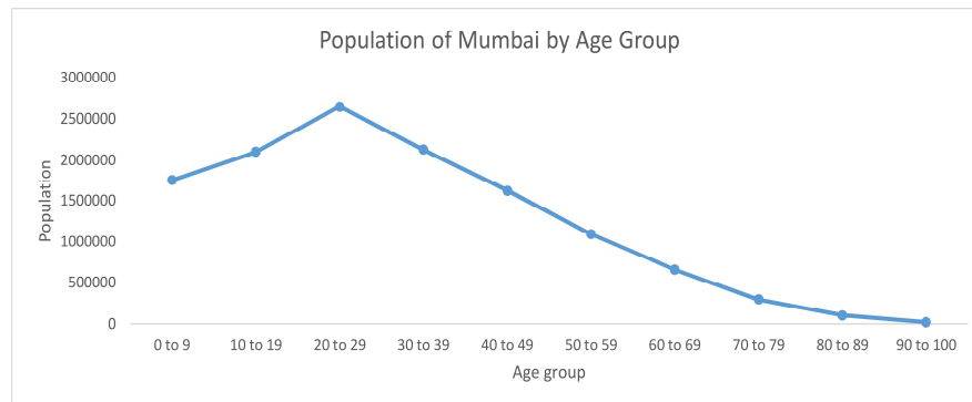
Figure 12: The distribution of the population according to the age category of Mumbai
