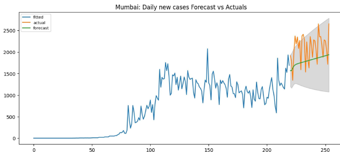
Figure 15: Compare actual and forecast data for daily new cases with an interval of 95%
