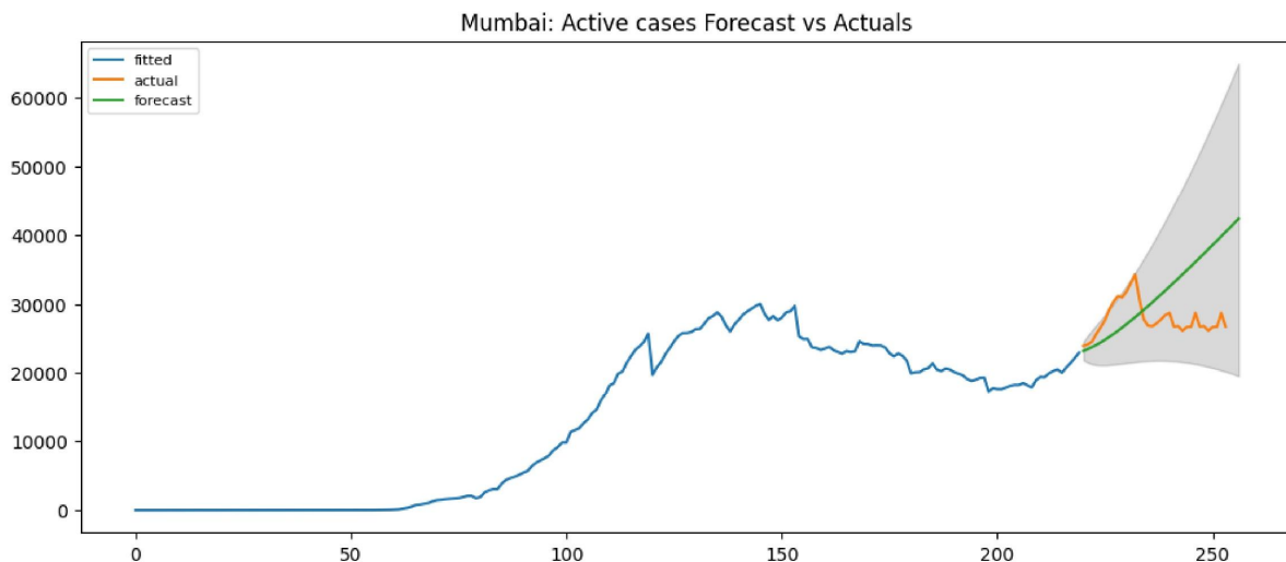
Figure 14: Compare the actual and forecast active case data with 95% interval
