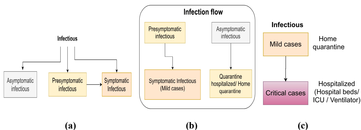
Figure 5: (a) Infectious cases categorization, (b) Infection flow, (c) Mild and severe infection flow
