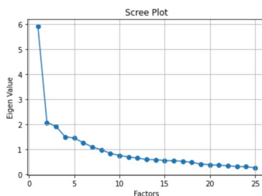
Figure 1: Scree-Plot for the EFA
