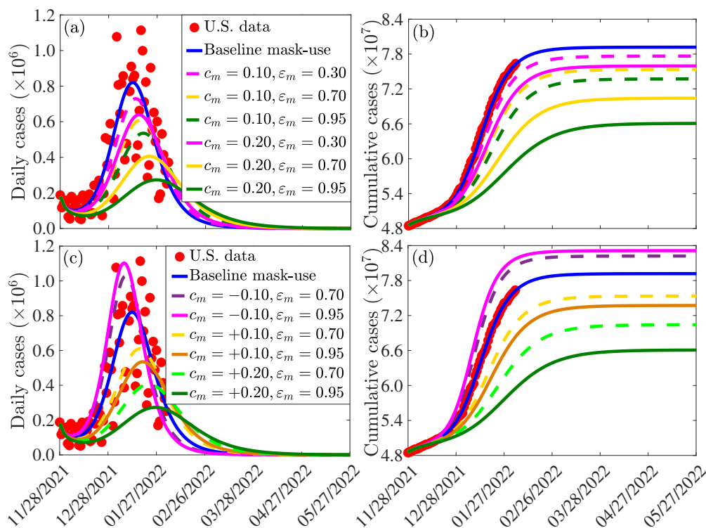
Figure 6: Simulations of the model (2.7) showing the incremental impact of mask coverage ( c_m ) and mask type (cloth masks, with \varepsilon_m = 0.3 ; surgical masks, with \varepsilon_m = 0.7 ; and N95 respirators, with \varepsilon_m = 0.95 ) on the daily ((a) and (c)) and cumulative ((b) and (d)) COVID-19 cases in the United States, as a function of time. The values of the other parameters used in these simulations are as given in Tables S3 and S4.
