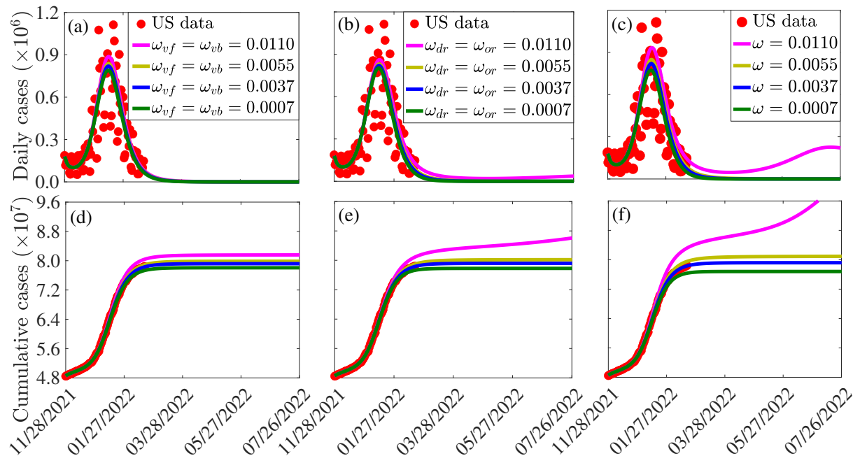
Figure 8: Simulations of the model (2.7), showing (a)-(c) new daily and (d)-(f) cumulative COVID-19 cases in the United States, as a function of time, for various values of the waning rate of (a) and (d) vaccine-derived immunity in fully-vaccinated and boosted individuals ( \omega_v = \omega_{vf} = \omega_{vb} ), (b) and (e) natural immunity for the Delta and Omicron variants ( \omega_r = \omega_{dr} = \omega_{or} ), and (c) and (f) both vaccine-derived and natural immunity ( \omega_{vr} = \omega_{vf} = \omega_{vb} = \omega_{dr} = \omega_{or} ). The durations for the waning of immunity were taken to be 3 months (i.e., \omega = 0.0110 per day), six months ( \omega = 0.0055 per day), nine months ( \omega = 0.0037 per day) and 48 months ( \omega = 0.0007 per day), respectively. The values of the other parameters used in these simulations are as given in Tables S3 and S4.
