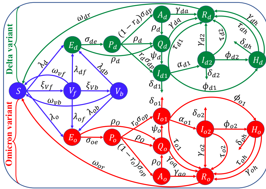
Figure 2: Flow diagram of the model (2.7). Although recruitment into the population and natural deaths occur (at the rate \Lambda and \mu , respectively), these rates are not illustrated in the flow diagram to make it less crowded and easier to follow. The state variables and parameters are described in Tables S1 and S2 of the supplementary material.
