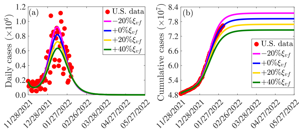
Figure 5: Simulations of the model (2.7) showing the effect of increases or decreases in fully-vaccinated vaccination coverage rate ( \xi_{vf} ) on the COVID-19 pandemic in the United States. (a) Daily cases, as a function of time, for various values of the fully-vaccinated vaccination coverage rate. (b) Cumulative cases, as a function of time, for various values of the fully-vaccinated vaccination coverage rate. The values of all other parameters used in these simulation are given by the baseline values in Tables S3 and S4.
