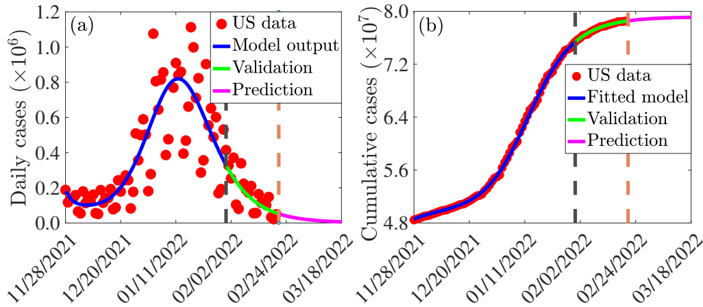
Figure 3: (a) Time series illustration of the least squares fit of the model (2.7), showing the model's output for the daily cases (blue curve) compared to the observed daily confirmed cases for the United States (red dots) from November 28, 2021 to January 31, 2022 (segment to the left of the dashed vertical black line). (b) Simulation result of the (2.7), showing cumulative COVID-19 cases for the United States as a function of time, using the fixed and estimated baseline parameter values given in Tables S3 and S4. The segment from February 1, 2022 to March 18, 2022 (i.e., solid green and magenta curves or the entire segment to the right of the dashed black vertical line) illustrates the performance of the model (2.7) in predicting the daily and cumulative cases in the United States.
