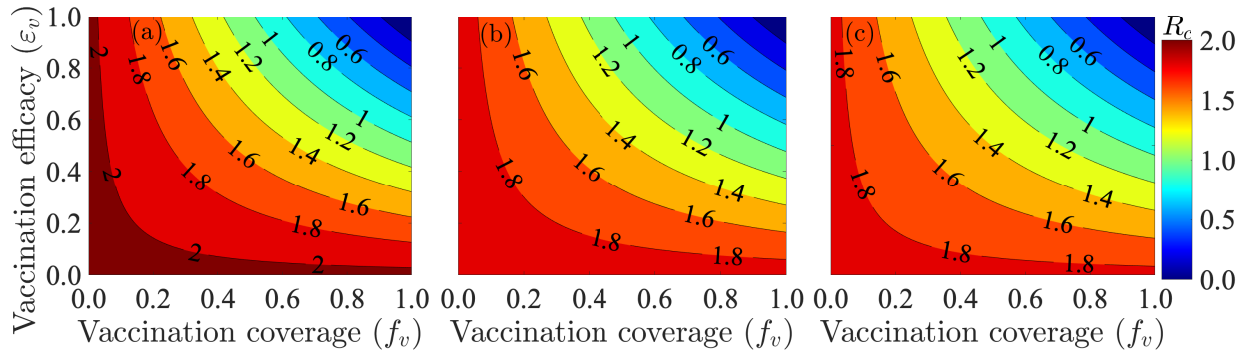
Figure 4: Contour plots of the control reproduction number of the model (2.7), \mathbb{R}_c , as a function vaccine coverage (i.e., proportion of fully-vaccinated individuals, f_v ) and cross-protective vaccine efficacy against the variants ( \epsilon_v = \min(\epsilon_{vf}, \epsilon_{vb}) ) for the case when (a) mask coverage is maintained at its baseline value, (b) surgical mask is prioritized and the coverage in its usage is increased by 10% from its baseline value, (c) N95 mask is prioritized and the coverage in its usage is increased by 10% from its baseline value. The values of all other parameters used in the simulations are as given by the baseline values in Tables S3 and S4.
