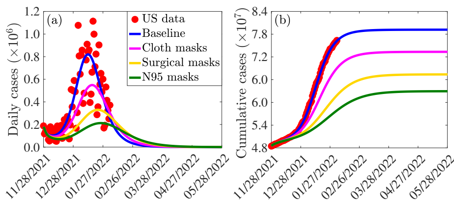
Figure 7: Simulations of the model (2.7), showing the combined incremental impact of mask coverage ( c_m ), mask type (cloth masks, with \varepsilon_m = 0.3 ; surgical masks, with \varepsilon_m = 0.7 ; and N95 respirators, with \varepsilon_m = 0.95 ) and fully-vaccinated vaccination coverage rate ( \xi_{vf} ) on the daily ((a)) and cumulative ((b)) COVID-19 cases in the United States, as a function of time. In these simulations, the mask and fully-vaccinated vaccination coverage rates are increased by 20% from their respective baseline values. The values of the other parameters used in these simulations are as given in Tables S3 and S4.
