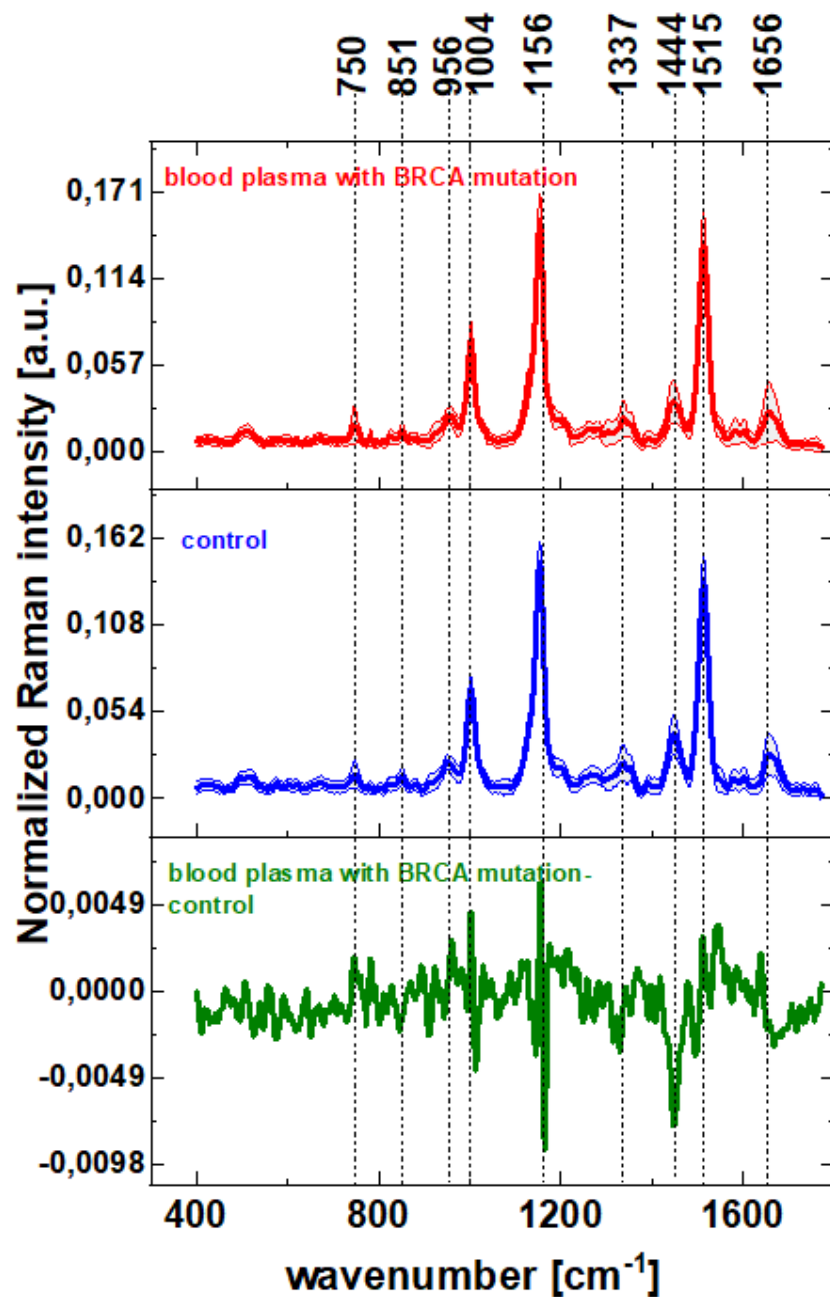
Fig 1 The normalized average Raman spectra typical for: (A) plasma from healthy patients (control) with SD (blue line), (B) plasma from patients with BRCA mutation with SD (red line), (C) the difference spectrum (blood plasma with BRCA - control) (green line)
