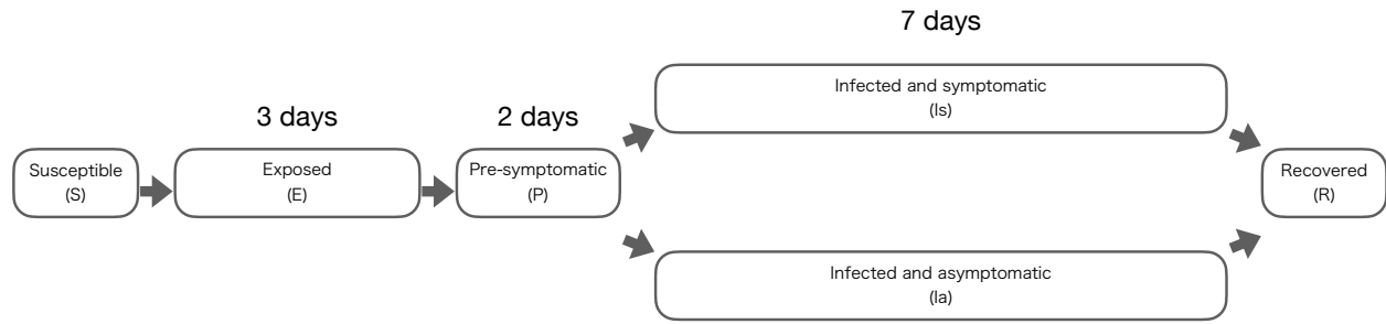
Figure 1: Discrete-time SEIR model used in the present study
