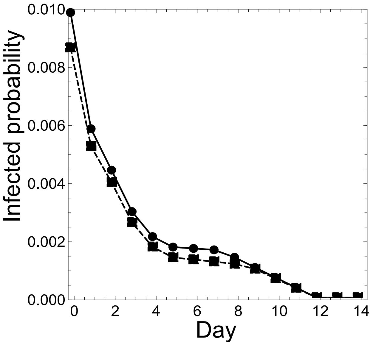
Figure 2: For x \neq 0 , the x -axis represents the day when an individual takes the second PCR test, and the y -axis the infection probability for an individual with a negative PCR test result on both day 0 and day x . For x = 0 , the corresponding y value represents the infection probability for an individual with a negative PCR test result on day 0. The dots show the infection probabilities for Case (i), and the squares for Case (ii). The solid and dashed lines connect the dots and squares, respectively.
