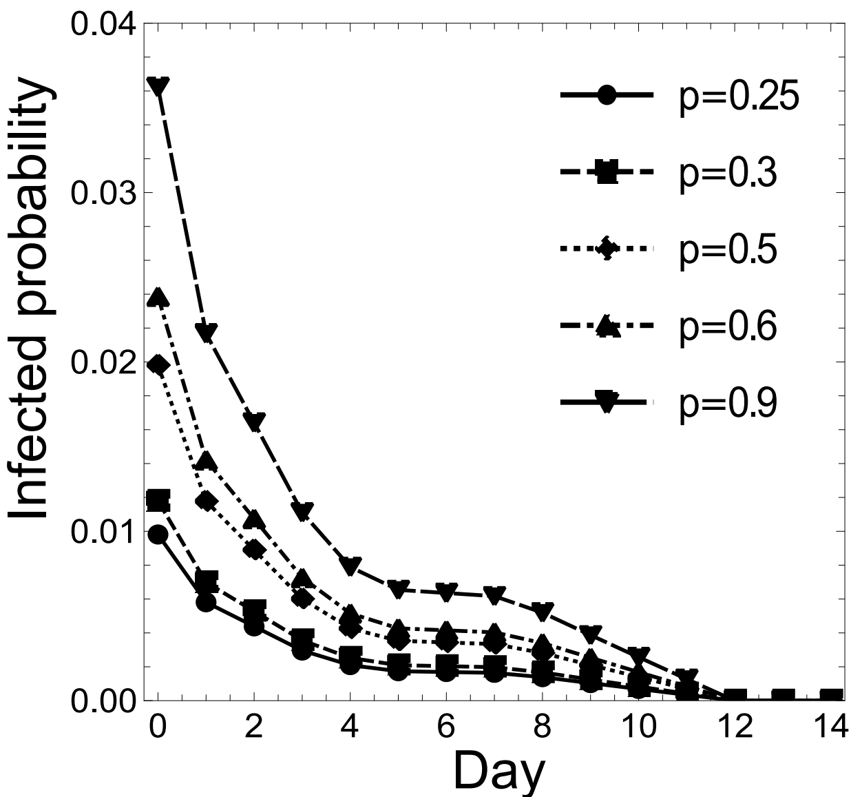
Figure 3: For x \neq 0 , the x -axis represents the day when an individual takes the second PCR test, and the y -axis the infection probability for an individual with a negative PCR test result on both day 0 and day x , for Case (i-CIs). For x = 0 , the corresponding y value represents the infection probability for an individual with a negative PCR test result on day 0, for Case (i-CIs). The dots, squares, diamonds, upward triangles, and downward triangles show the infection probabilities for p = 0.25, 0.30, 0.50, 0.60, 0.90 , respectively, for Case (i-CIs); and the solid, short-dashed, dotted, dash-dotted, and long-dashed lines connect the dots, squares, diamonds, upward triangles, and downward triangles, respectively.
