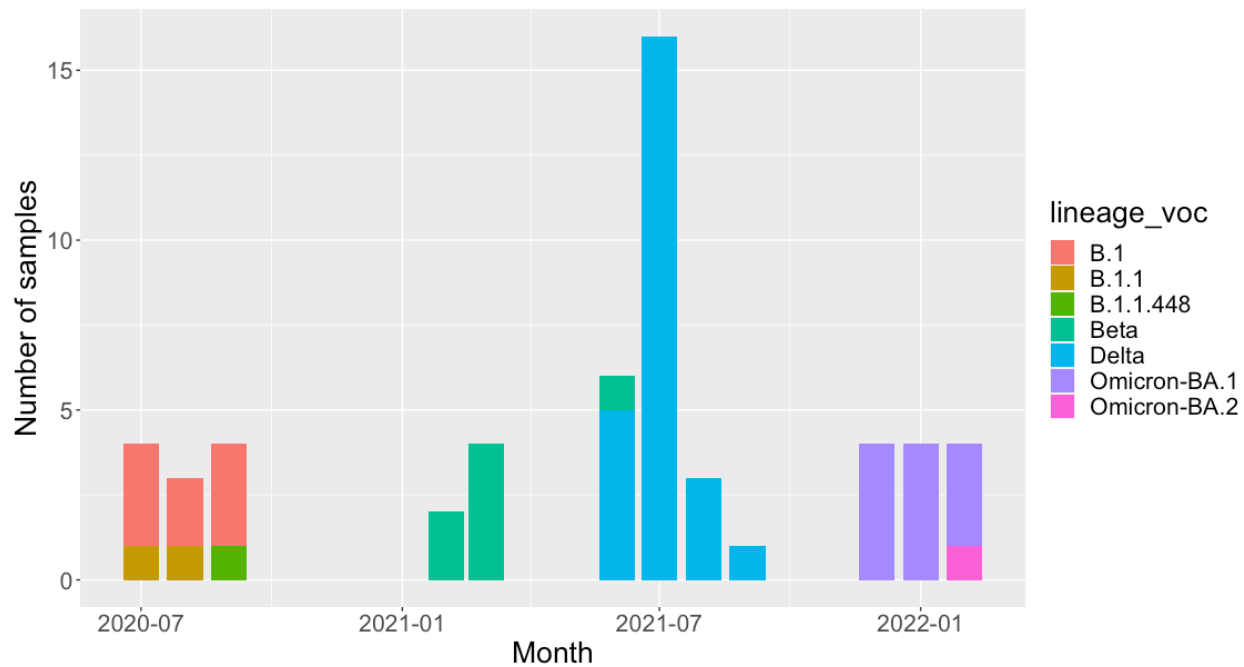
238 Figure 2: The monthly number of each lineage or VOC identified in patients in our cohort.
