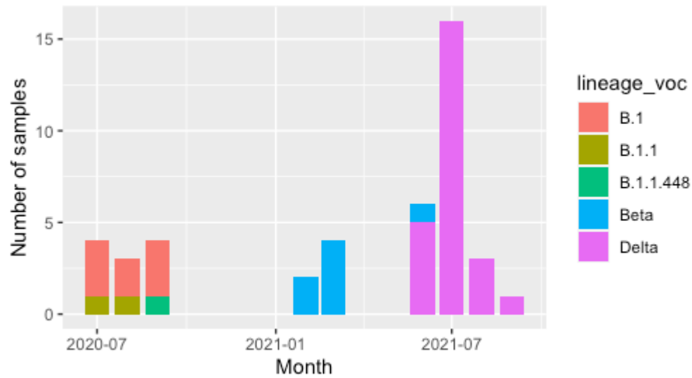
Figure 2: A histogram of the monthly number of each lineage or VOC identified in patients in our cohort.
