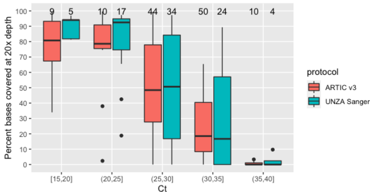
Figure 1: Relationship between PCR Ct value and the percentage of the SARS-CoV-2 reference genome covered to at least 20x depth. The number at the top of each column is the number of samples for the two protocols in each bin of the box plot.
