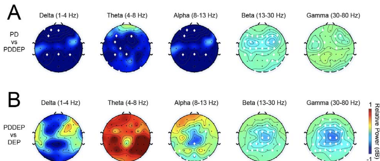
Figure 1: Scalp topography of relative EEG power in PD patients with depression . A) Relative power in PD patients with depression (PDDEP) compared to PD patients without depression for delta (1-4 Hz), theta (4-8 Hz), alpha (8-13 Hz), beta (13-30 Hz), and gamma (30-80 Hz). B) Relative power in PDDEP compared to non-PD patients with depression (DEP). Electrodes are indicated by black dots; electrodes with significant differences between groups via ranksum testing are shown with white diamonds. Data from 18 PD, 18 PDDEP and 12 DEP.
