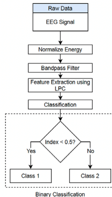
Figure 2: LEAPD Classification approach: Flow chart of classification.
