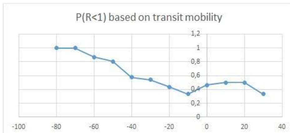
Figure 7. Estimated probability of R below spread levels based on transit station mobility.
