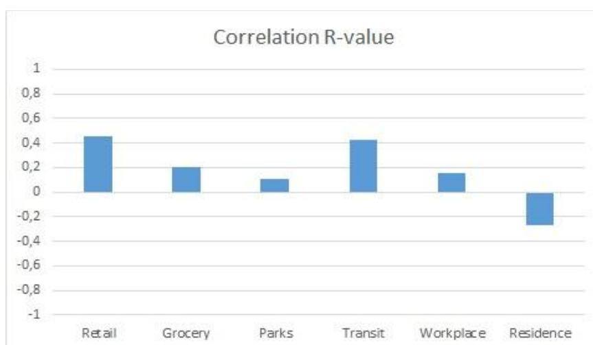
Figure 4. Correlations sector mobilities and reproduction.
