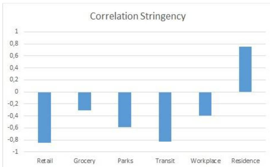
Figure 3. Correlations Stringency – Mobility.
