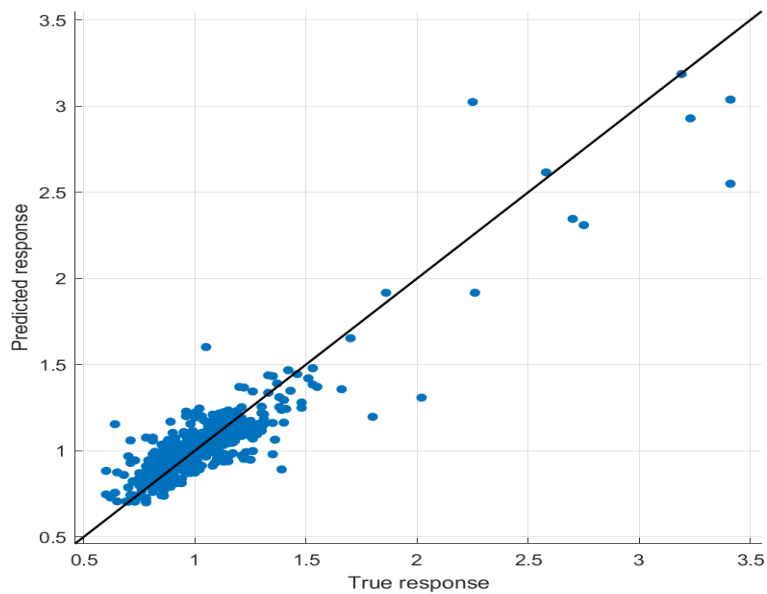
Figure 5 Model fit of GPR model.
