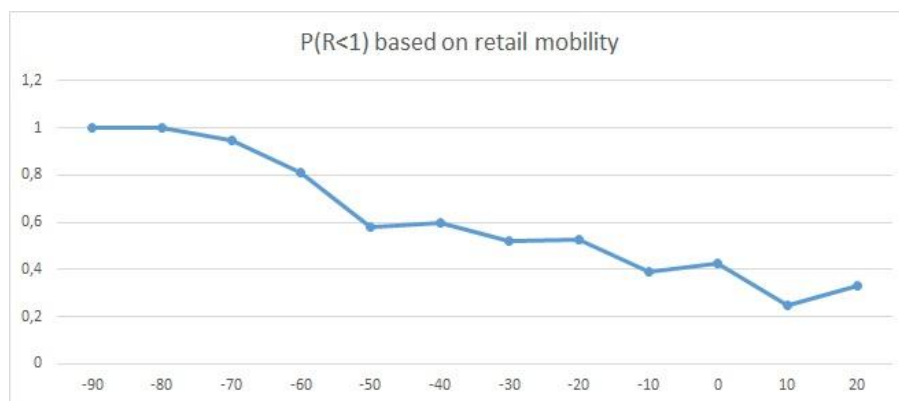
Figure 6. Estimated probability of R below spread levels based on retail mobility.
