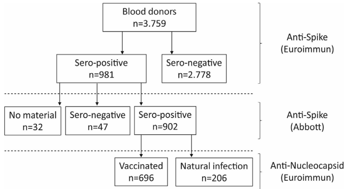
Figure 1: Flow-chart illustrating the methodological design of the present seroprevalence study. A total of 3,759 blood donors were tested for anti-SARS-CoV-2 antibodies over a one-year period. Initial positive samples were validated using a second test. To differentiate between vaccinated and convalescent blood donors among the positive samples, a final assay was performed to detect antibodies against the nucleocapsid, only being expressed by convalescents.
