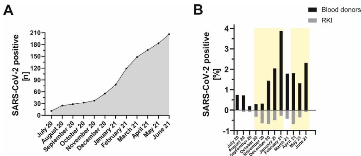
Figure 2: Monthly anti-SARS-CoV-2 antibody detection in the period between July 2020 and June 2021 in blood donors residing in the three German federal states North Rhine-Westphalia, Lower Saxony and Hesse. A: Cumulative illustration of anti-SARS-CoV-2 seropositives by month. B: Comparison of percentage anti-SARS-CoV-2 positivity rate among donors (seroprevalence, black bars) with officially reported data from the Robert-Koch-Institute [4] (PCR detection, grey bars). The light-yellow areas symbolize the second- and third corona wave in Germany.
