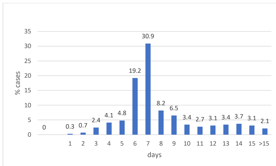
Figure 2– Time to recovery after PCR positivity in Omicron cases
