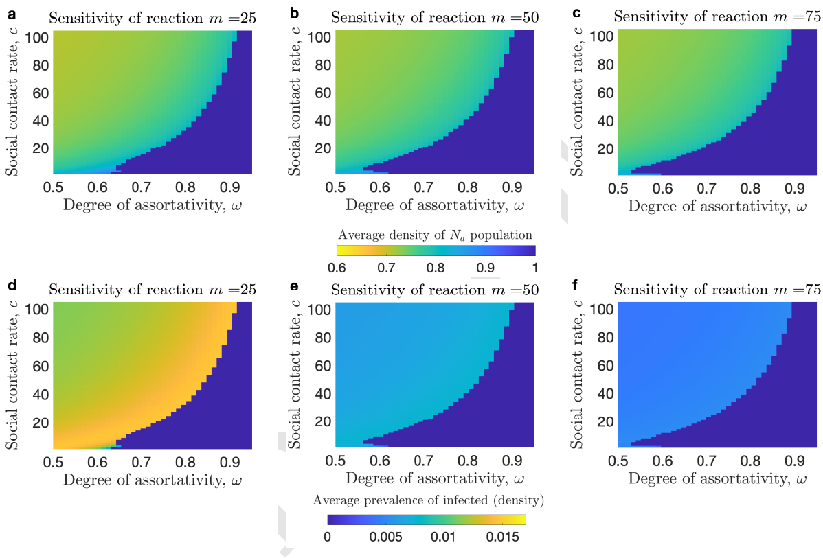
Fig. 9. Impact of social contact rate and assortativity on the average endemic prevalence of infectious cases and average long-term opinion distribution. We consider the dynamics of the SIS system. a , b , and c show heat maps of the long term average density of the N_a population. d , e , and f show heat maps of the long term average infection prevalence. If the epidemic dynamics are periodic, then the average is taken over a period. a and d show scenarios with sensitivity of reaction to prevalence given by m = 25 . b and e show scenarios with sensitivity of reaction to prevalence given by m = 50 . c and f show scenarios with sensitivity of reaction to prevalence given by m = 75 . The dark blue region in the top row and dark blue region in the bottom row denote the outcome where the population switched to opinion a and the disease becomes extinct. The infection rate of N_b individuals was set \beta_b = 1.5 .
