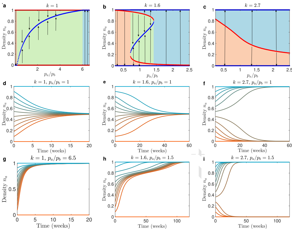
Fig. 3. Opinion competition dynamics for saturating and sigmoidal switch rate functions. The upper row shows bifurcation diagrams of n_a as a function of p_a/p_b . For a a saturating switch rate function; b and c sigmoidal switch rate functions. Red lines: unstable equilibria, blue lines: stable equilibria. Orange area: basin of attraction for the equilibrium with opinion b dominating; blue area: basin of attraction for the equilibrium where opinion a dominates; green area: basin of attraction of a stable co-existence equilibrium. d-i Temporal dynamics of n_a for different switch rate functions and ratios p_a/p_b . In all panels \theta_a = \theta_b = 5 .
