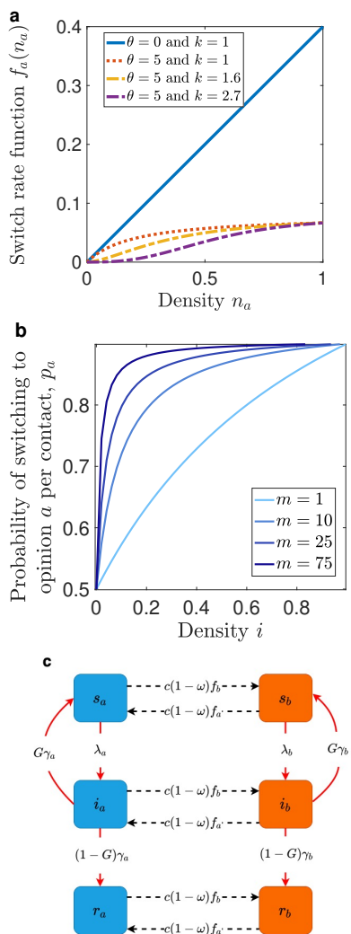
Fig. 1. Coupling of opinion dynamics and infection transmission dynamics. a Switch rate function to opinion a depending on density n_a . For \theta = 0 and k = 1 the switch rate is linear (blue); for \theta > 0 and k = 1 the switch rate is saturating (red); for \theta > 0 and k > 1 the switch rate is sigmoid (yellow and violet). b Per contact probability of switching to opinion a for different values of m as a function of the density of infected individuals, i . c Flowchart of coupled opinion and infection transmission model for two types of infectious diseases: SIS model ( G = 1 ) and SIR model ( G = 0 ); black dashed arrows denote opinion transitions, red solid arrows denote epidemiological transitions.
