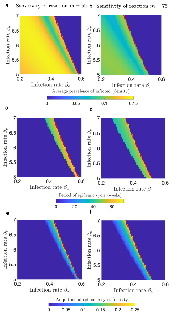
Fig. 10. Impact of assortativity and sensitivity of reaction to the prevalence of infectious cases on the appearance of periodic epidemic dynamics. We consider the dynamics of the SIS system. a and b show heat maps of the average prevalence. If the epidemic dynamics are periodic, then the average is taken over a period. c and d show heat maps of the period of the epidemic cycle. The period is equal to zero if the dynamics are stationary. e and f show heat maps of the amplitude of epidemic cycle. The amplitude is zero if the dynamics are stationary. a , c , and e show scenarios with sensitivity of reaction to prevalence given by m = 50 . b , d , and f show scenarios with sensitivity of reaction to prevalence given by m = 75 . The dark blue region above the red line denotes the outcome where the population switched to opinion a and the disease becomes extinct. The probability of switch to opinion a when no infectious cases are present is fixed p_a(0) = 0.28 , the probability of switch to opinion a when the whole population is infected is fixed to p_a(1) = 0.6 . Social contact rate is fixed c = 10 .
