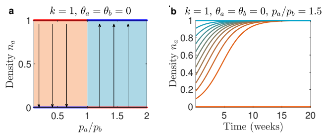
Fig. 2. Opinion competition dynamics for a linear switch rate function. We consider opinion dynamics in the disease-free population. a Bifurcation diagram of n_a as a function of p_a/p_b . Red lines: unstable equilibria, blue lines: stable equilibria. Orange area: basin of attraction of the mono-belief b equilibrium, blue area: basin of attraction of the mono-belief a equilibrium. b Temporal dynamics of n_a for p_a/p_b = 1.5 . All solutions where initially both opinions are present converge to the state where opinion a dominates.
