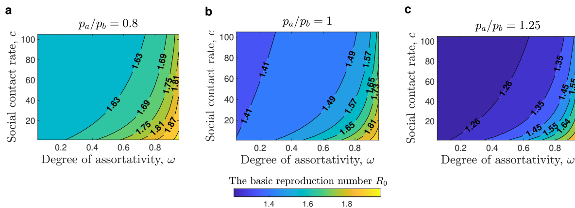
Fig. 4. Impact of mixing patterns on basic reproduction number R_0 . a , b , and c show contour maps of R_0 as a function of the social contact rate c and the assortativity \omega . a For p_a/p_b = 0.8 the initial distribution of opinions is (s_a(0), s_b(0)) = (0.35, 0.65) . b For p_a/p_b = 1 we have (s_a(0), s_b(0)) = (0.5, 0.5) . c For p_a/p_b = 1.25 we have (s_a(0), s_b(0)) = (0.65, 0.35) . The infection rate of susceptible individuals holding opinion a is fixed \beta_b = 2 , the value used to investigate the dynamics for the SIR system. For the same set of figures with \beta_b = 1.5 , the value used to investigate the dynamics of the SIS model, see Figure S2 in SI.
