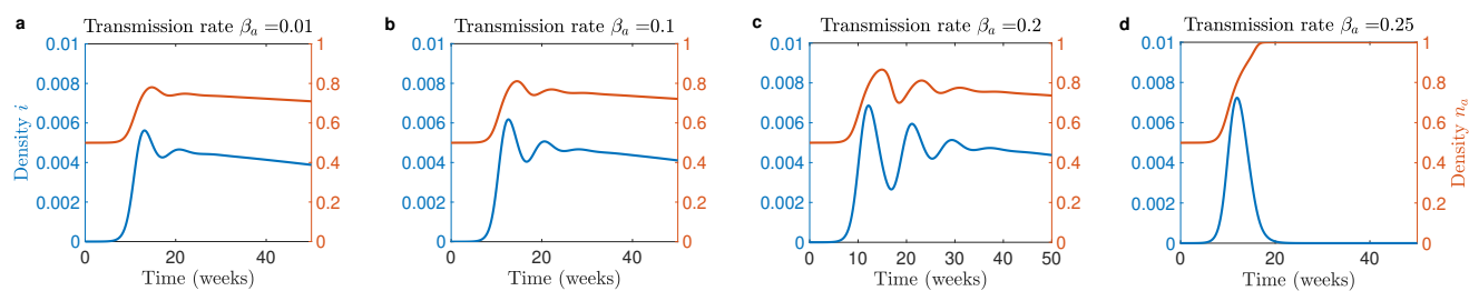
Fig. 8. Temporal dynamics with multiple epidemic peaks resulting from feedback between disease dynamics and opinion dynamics. We consider the dynamics of the SIR system. Panels show time series of infection prevalence, and of the density of the N_a population, n_a for different values of infection rate \beta_a . The social contact rate was fixed at c = 40 , the upper bound of the probability of switching to opinion a was set to p_a(1) = 1 , the sensitivity parameter m was set to m = 75 , the infection rate of N_b individuals was set to \beta_b = 4.15 , and the assortativity degree is fixed \omega = 0 .
