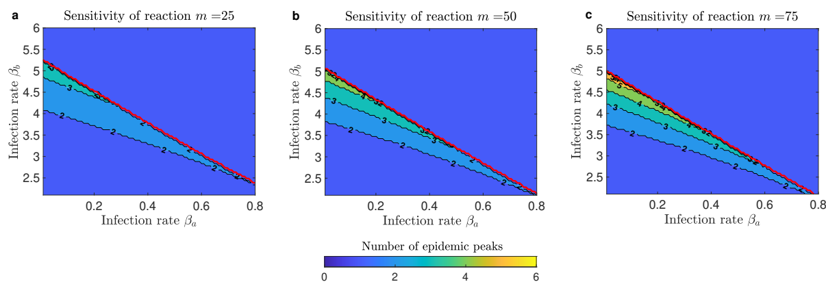
Fig. 7. Regions of multiple epidemic peaks resulting from feedback between disease dynamics and opinion dynamics. We consider the dynamics of the SIR model. a , b , and c are contour plots of the number of prevalence peaks for different values of infection rates \beta_a and \beta_b for different sensitivity m of the population to increasing prevalence: a m = 25 , b m = 50 , and c m = 75 . The social contact rate is fixed at c = 40 , and the probability of switch to opinion a per contact when the entire population is infected is fixed p_a(1) = 1 , and the assortativity degree is fixed \omega = 0 . The area above the red curve denotes the outcome where the population switched to opinion a . As m increases this region expands.
