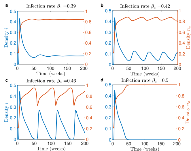
Fig. 11. Sustained oscillatory dynamics resulting from feedback between disease dynamics and opinion dynamics. We consider the dynamics of the SIS system. Panels show time series for the prevalence of infectious cases and density of N_a population, n_a for different values of infection rate of N_a population, \beta_a . The contact rate for information exchange is fixed c = 10 , the probability of switch to opinion a when no infectious cases are present is fixed p_a(0) = 0.28 , the probability of switch to opinion a per contact when the whole population is infected is fixed p_a(1) = 0.6 , the constant that controls the growth of the switch rate to opinion a is fixed m = 75 , and the infection rate of N_b individuals is fixed to \beta_b = 5.5 .
