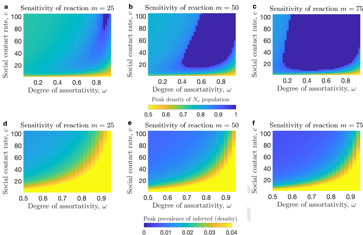
Fig. 5. Impact of social contact rate and assortativity on epidemic dynamics. We consider the dynamics of the SIR system for three scenarios for the sensitivity of the population to increasing prevalence of infection as denoted by parameter m , m = 25 for a and d , m = 50 for b and e , and m = 75 for c and f . a , b , and c show heat maps of the peak density of the N_a population; in the dark blue region the population converts to opinion a . d , e , and f show contour maps of the peak prevalence.
