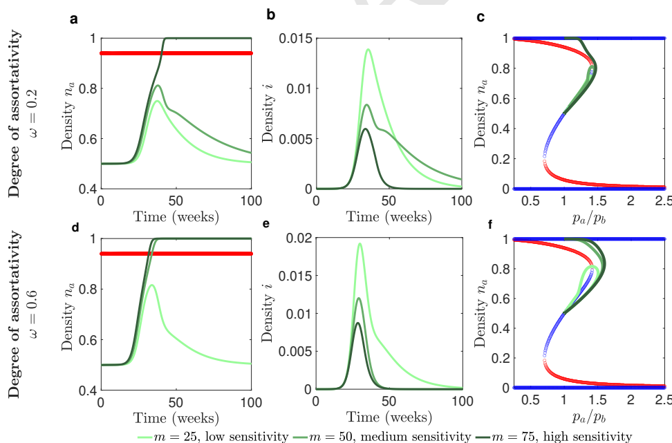
Fig. 6. Impact of assortativity on the population adopting opinion a . We consider the dynamics of the SIR system. a and d show density of N_a population n_a in time, b and e show the prevalence of infectious cases in time, c and f show phase diagrams for three different solutions overlaid over a bifurcation diagram for density of N_a population, n_a , component of permanent distributions. a , b , and c are plotted for degree of assortativity \omega = 0.2 , a , b , and c - for \omega = 0.6 . Social contact rate is fixed c = 40 .
