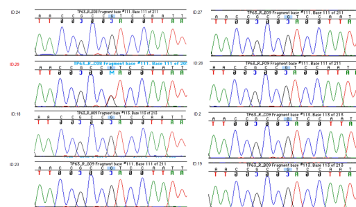
Fig. 1. Sanger sequencing results of TP63 mutation in all available family members.
