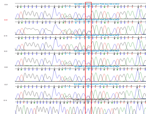
Fig. 2. Sanger sequencing results of HLA-DRB5 variant in all available family members
