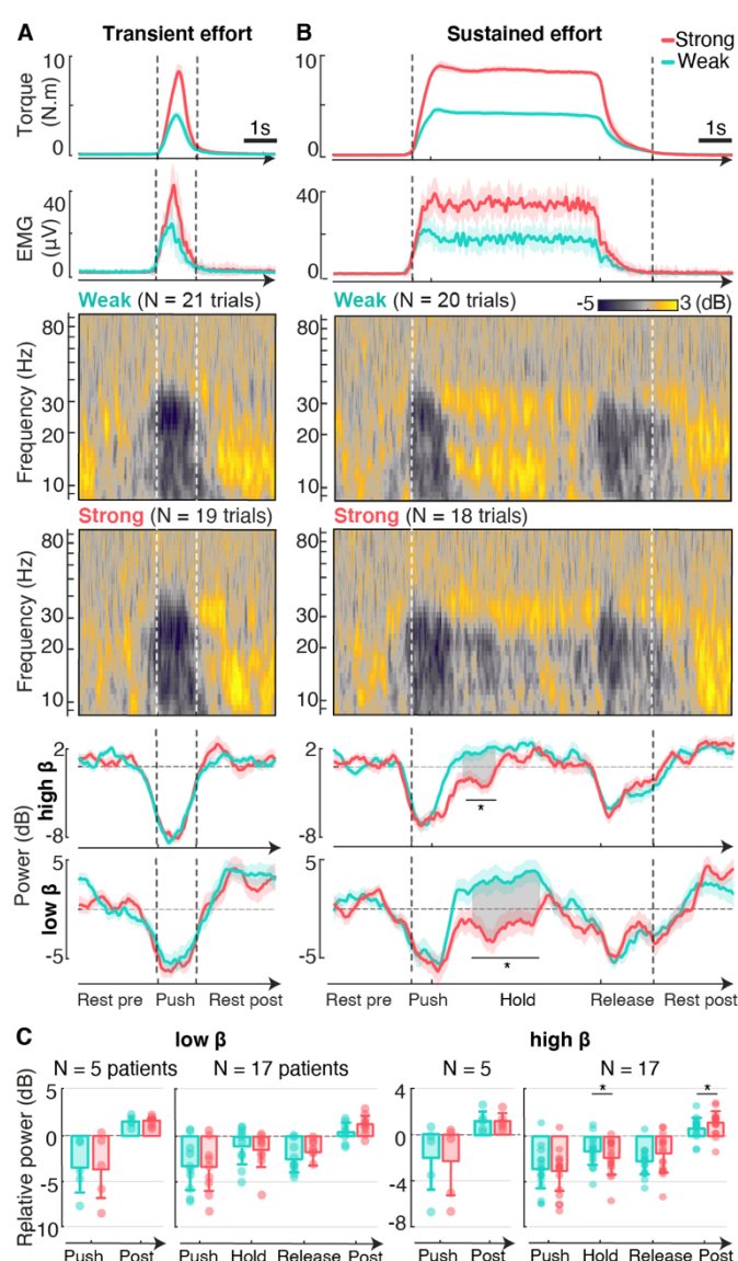
Figure 2 | STN encodes muscle activation dynamics. Patients performed an isometric knee extension task with two levels of force (weak 33% of maximal voluntary contraction, strong 66%). (A) Task involving a transient effort (participant P1). Average traces of torque and knee extensor muscle envelope (mean \pm SD), average spectrograms of the contralateral STN normalized to baseline (rest pre-movement, defined as 2.5s before the onset of effort) and traces of low- and high- beta power (mean \pm SD). (B) Same plots for a task involving a sustained effort. Shaded areas show significant differences in band-power when tasks performed with a weak and a strong force (Monte-Carlo cluster comparison). (C) Barplots of low- and high-beta power (mean \pm SD) for both tasks. N = 17 patients performed the sustained task, only N = 5 of them performed the transient task. Low-beta was identified in all participants, and high-beta in 4/5 and 10/17 participants respectively. * p < 0.05 paired t-test with Bonferroni correction. No difference was found between levels of force for the transient task at the group level (two-way ANOVA, n=5 : Effect of time window: df=2 , low beta: F=2.64 , p=0.09 ; high beta: F=8 , p=0.002 . Effect of force: df=1 , low beta: F=0.04 , p=0.83 ; high beta: F=0.02 , p=0.90 ). Within participants: 5/5 (exhibiting low beta) and 4/5 (high beta) showed a significant effect of the time window (Two-way unbalanced ANOVA); 1/5 (low beta) and 0/5 had an effect of force. For the sustained task: 9/10 (low beta) and 17/17 (high beta) showed a significant effect of the time window. 3/10 (low-beta) and 7/17 (high-beta) had a significant effect of force.
