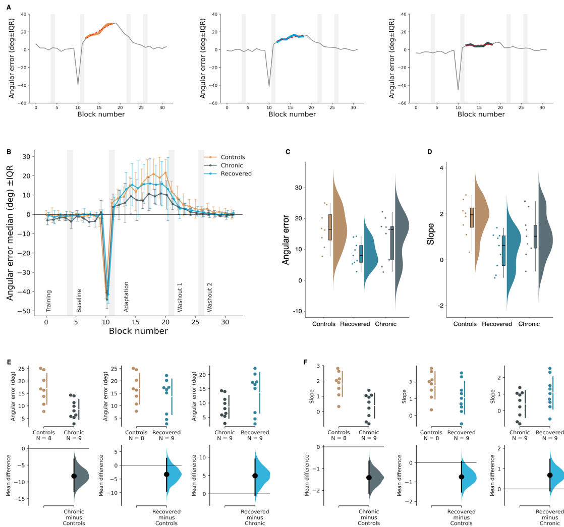
Figure 2. Implicit motor adaptation. (A): Slope fit during the Rotation+Strategy phase for one representative subject per group. (B): Directional aiming errors throughout the phases of the VMR task. Vertical shaded areas indicate the first 8-trials bin of each phase. The horizontal line shows the target direction (i.e., no directional error, 0° error). Each point represents the median of the errors of each block of 8 trials. Error bars indicate IQRs. (C-D): Group comparison of median angular errors and regression line fits during the Rotation+Strategy phase. (E-F): Pairwise comparisons of median of errors and regression line fits during Rotation+Strategy phase. *: p < 0.05 ; **: p < 0.01 ; NS: not significant. Error bars indicate the IQR.
