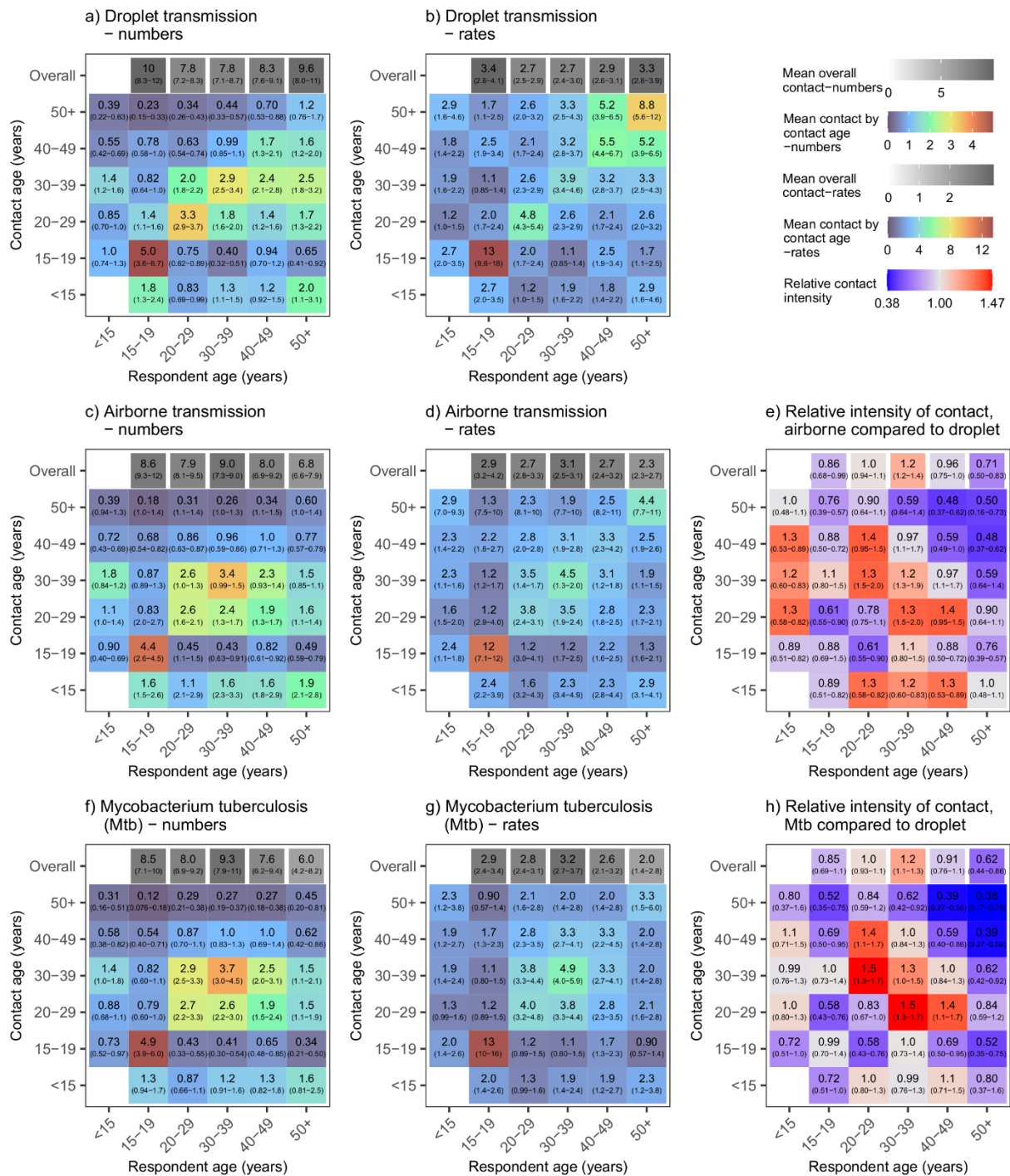
Figure 4. Age mixing matrices relevant for droplet transmission, non-saturating airborne transmission, and Mycobacterium tuberculosis transmission, for Western Cape. Graphs a, c, and f show absolute contact intensities between respondents and contacts in each age group. Graphs b, d, and g show age intensities of contact between each member of each age group. Graphs e and h show intensities for airborne infections and Mtb compared to
