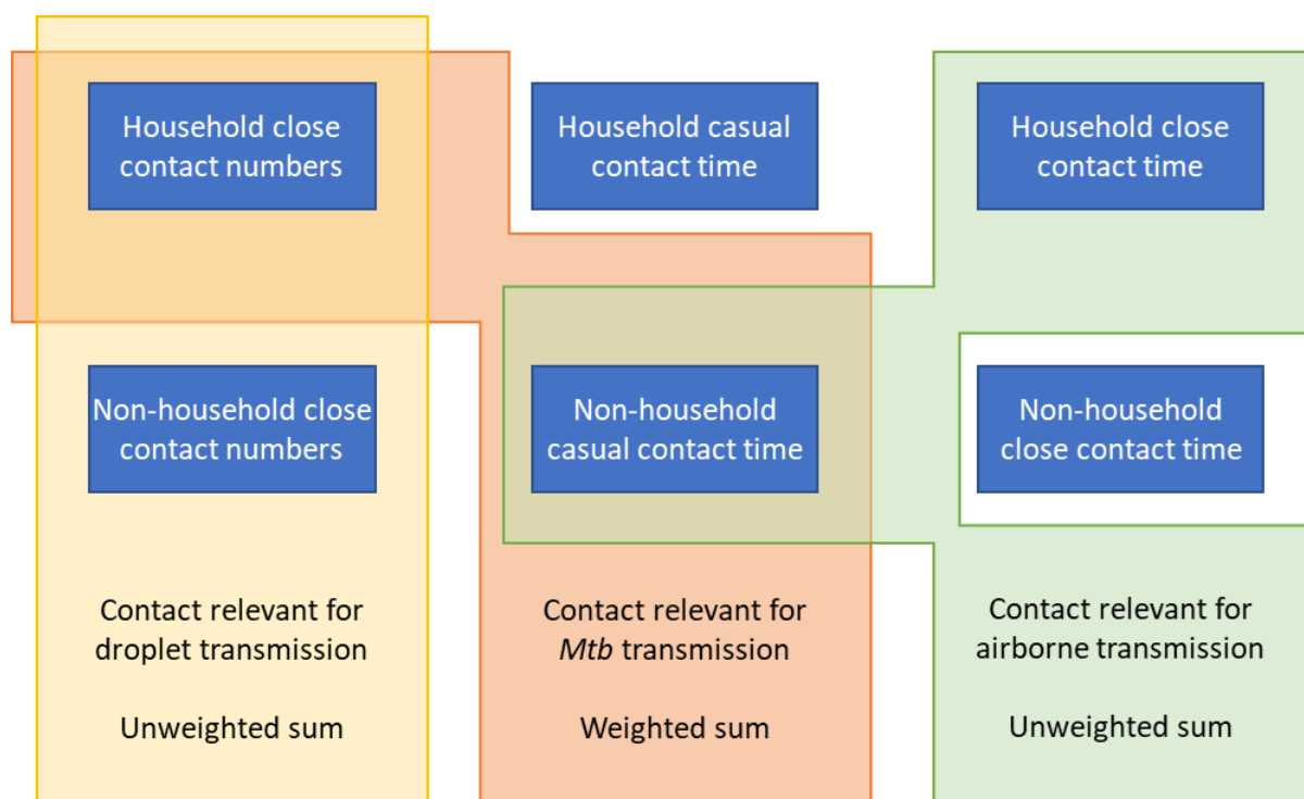
Figure 1. Summary of data used to estimate age-mixing matrices. Diagram showing how age-mixing matrices relevant for the transmission of droplet infections, airborne infections, and Mycobacterium tuberculosis were estimated using empirical data on close contact numbers, close contact time, and casual contact time.
