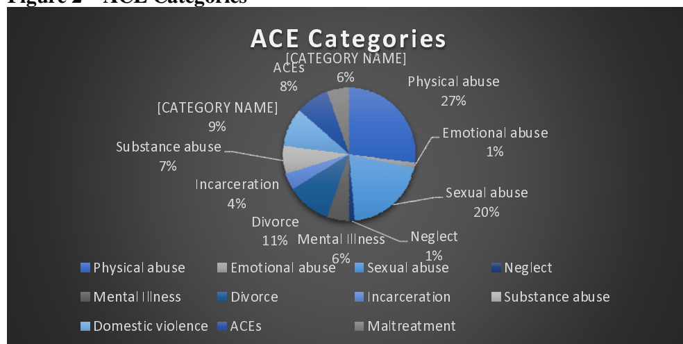
Figure 2 – ACE Categories
