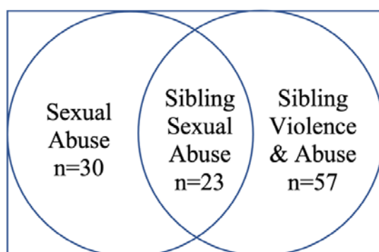
Figure 3 – Venn Diagram
