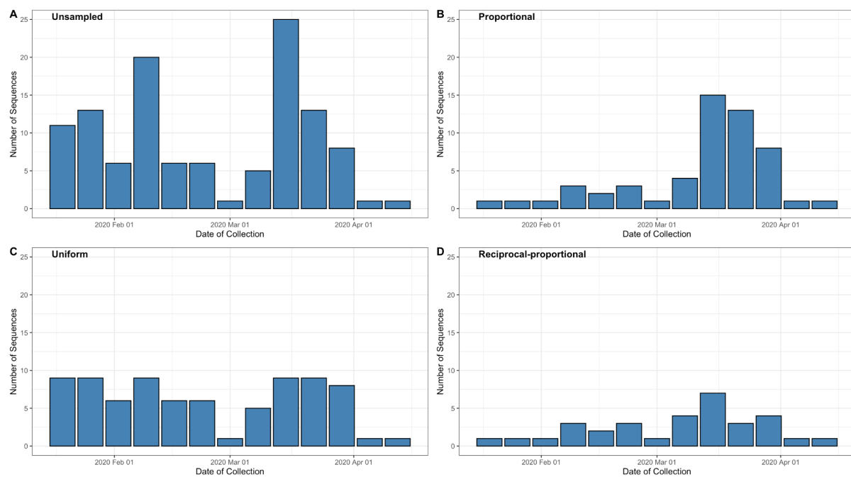
Supplementary Figure 2: Number of sequences for each week and sampling scheme for Hong Kong dataset.
