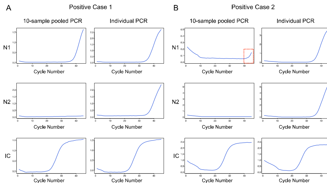
Figure 1. PCR amplification curves for positive case 1 (A) and positive case 2 (B). Upper panel, N1; middle panel, N2; lower panel, human internal control (IC) gene. Left column of each panel, 10-sample pools; right column of each panel, individual samples.
