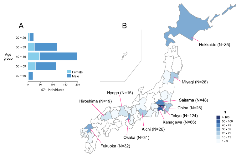
Figure 3. Characteristics of survey participants. (A) Age group distribution with males (blue) and females (light blue). (B) Locations at the time of screening, showing prefectures with more than 10 participants.
