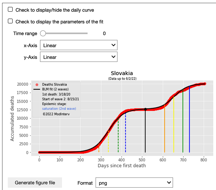
Figure 6: Output of the numerical fit of the epidemic curve (Deaths) for the selected country (Slovakia).
