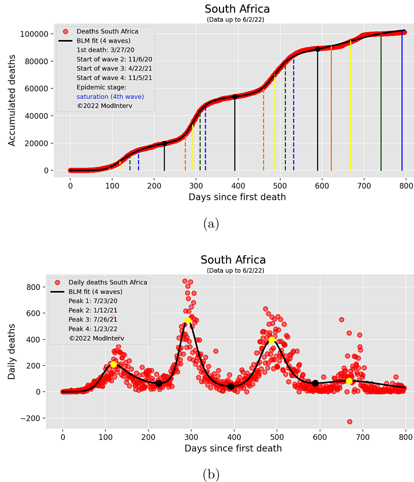
Figure 10: Cumulative (a) and daily (b) curves (empirical data and theoretical fit) for deaths attributed to COVID-19 in South Africa up to June 2, 2022.
