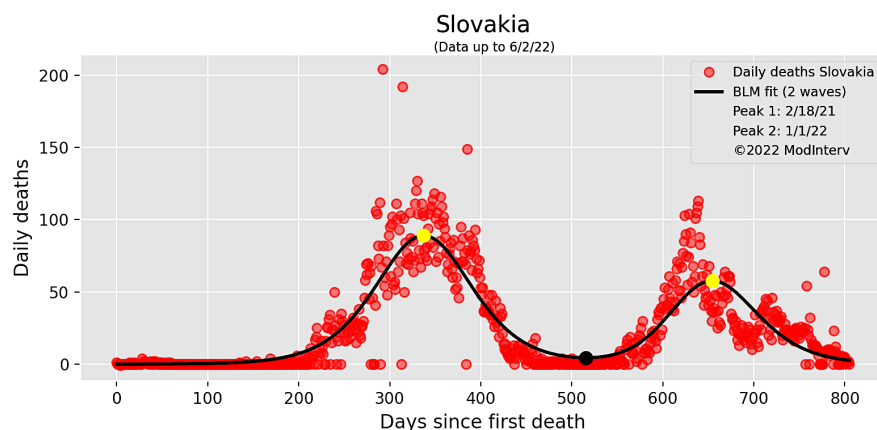
Figure 7: Daily curves (empirical and theoretical) corresponding to the cumulative curves shown in Fig. 6.
