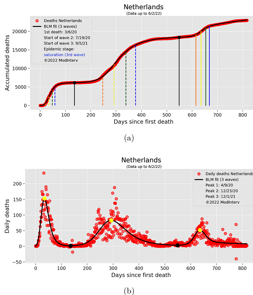
Figure 9: Cumulative (a) and daily (b) curves (empirical data and theoretical fit) for deaths attributed to COVID-19 in the Netherlands up to June 2, 2022.
