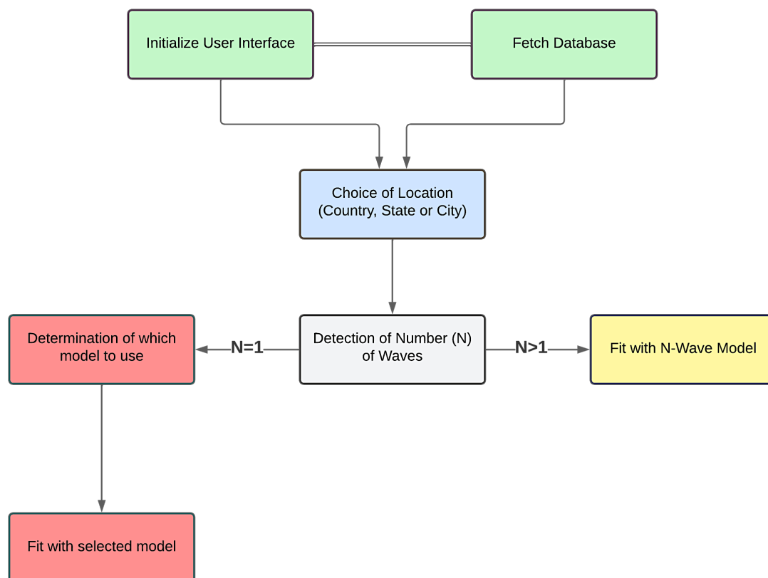
Figure 3: Simplified schematic description of the workflow of the software behind the app ModInterv .
