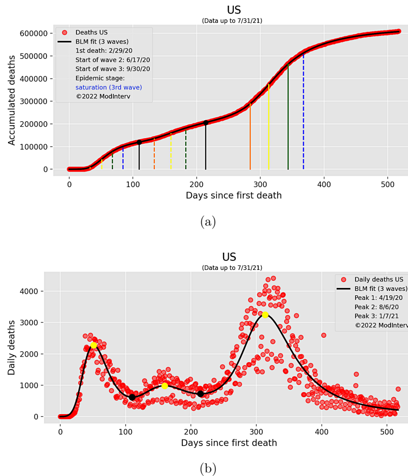
Figure 11: Cumulative (a) and daily (b) curves (empirical data and theoretical fit) for deaths attributed to COVID-19 in the USA up to a time (July 31, 2021) when there were three waves of infection.
