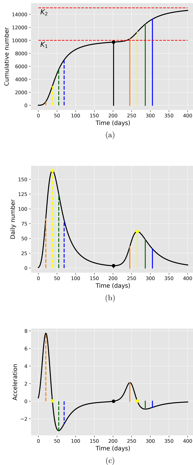
Figure 1: (a) Schematic of a cumulative epidemic curve with two waves of infection, illustrating the five main acceleration regimes in each wave, as separated by the colored dashed (solid) vertical lines for the first (last) wave. The black dot and the solid black line descending from it indicate the beginning of the second wave. (b) Velocity and (c) acceleration curves, corresponding to the first and second derivatives, respectively, of the cumulative curve shown in (a). The yellow circles in (b) indicate the wave peaks.
