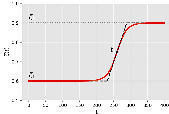
Figure 2: Time dependence of the generic parameter \zeta(t) of the N -wave model, as defined by the logistic function given in (2), for the case of N = 2 (two waves). The dashed line represents the linear approximation to the logistic function, where the inclined straight line meets the upper and lower horizontal lines at the points t_1 \pm 2/\rho_1 , where t_1 and \rho_1 are respectively the transition time and rate between the two plateaus.
