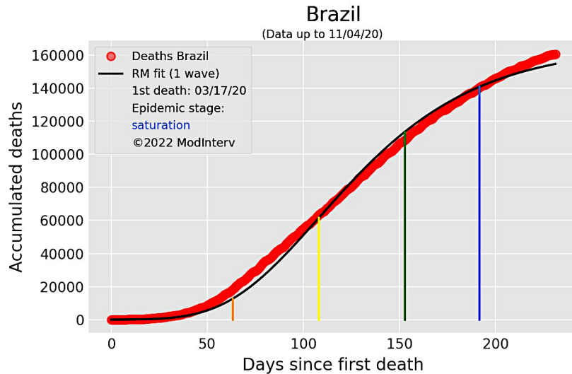
Figure 11: Numerical fit for the cumulative number of deaths in Brazil up to a time (11/04/2020) when there was only one wave of infection.
