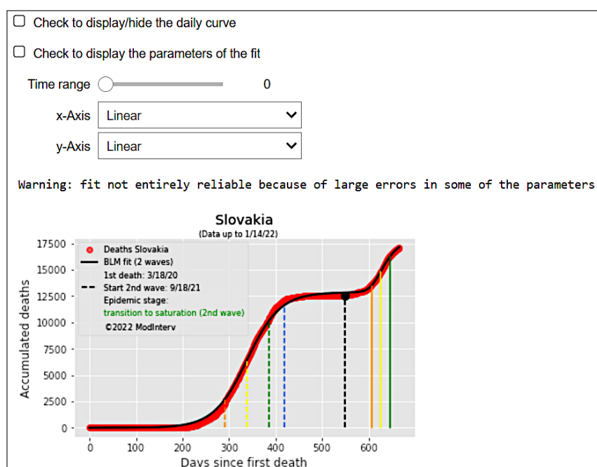
Figure 8: Output of the numerical fit of the epidemic curve (Deaths) for the selected country (Slovakia).
