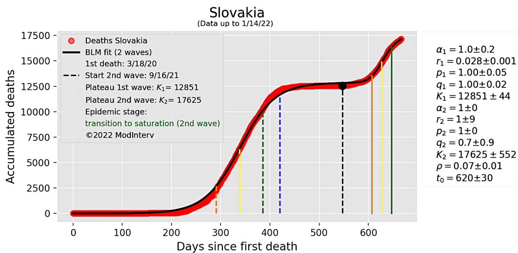
Figure 10: Detailed output of the numerical fit shown in Fig. 8, indicating the values of the fitted parameters with their respective errors.
