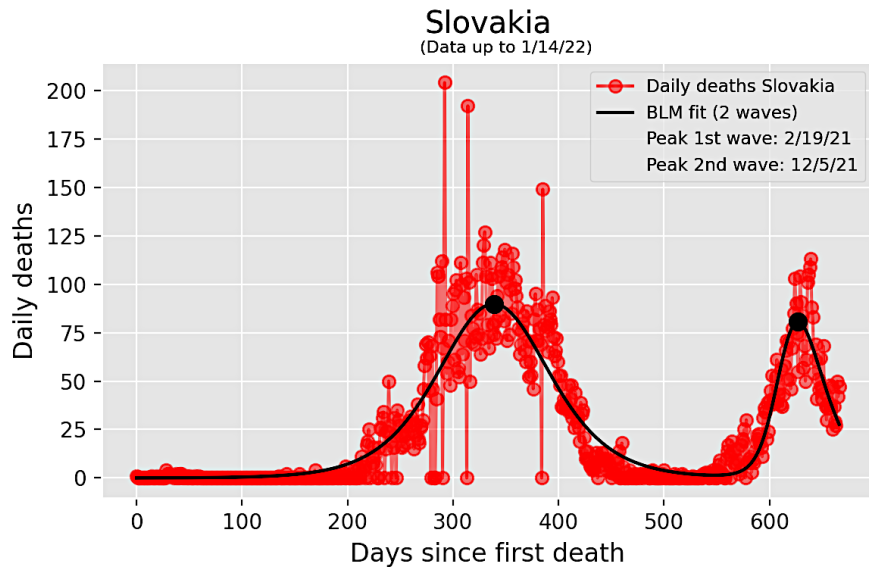
Figure 9: Daily curves (empirical and theoretical) corresponding to the cumulative curves shown in Fig. 8.
