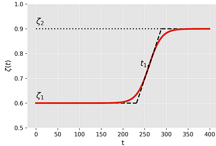
Figure A.12: Time dependence of the generic parameter \zeta(t) of the two-wave model, as defined by the logistic function given in (B.2). The dashed line represents the linear approximation to the logistic function, where the inclined straight line meets the upper and lower horizontal lines at the points t_1 \pm 2/\rho_1 , where t_1 and \rho_1 are respectively the transition time and rate between the two plateaus; see text.
