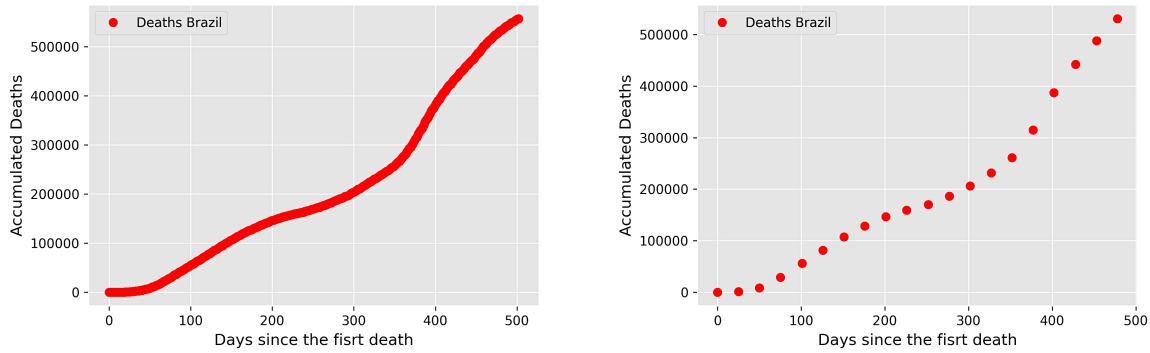
(a) Cumulative Deaths curve for Brazil up to 08/03/21.
