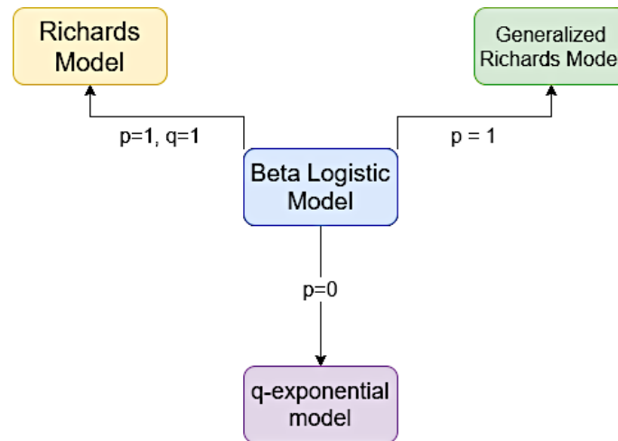
Figure 3: Schematic figure indicating the q -exponential, Richards and generalized Richards models as particular cases of the beta logistic model.
