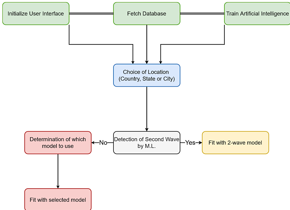
Figure 4: Simplified schematic description of the workflow of the software behind the app ModInterv.
