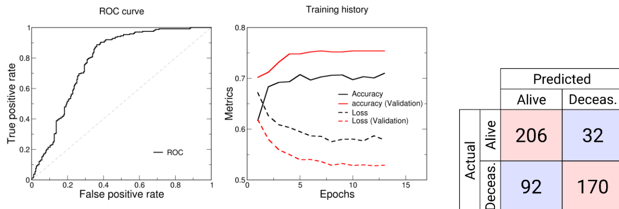
Figure 3. Patient outcome prediction by DL classification model. (left) ROC curve and training history of the best classification model. (right) The confusion matrix.
