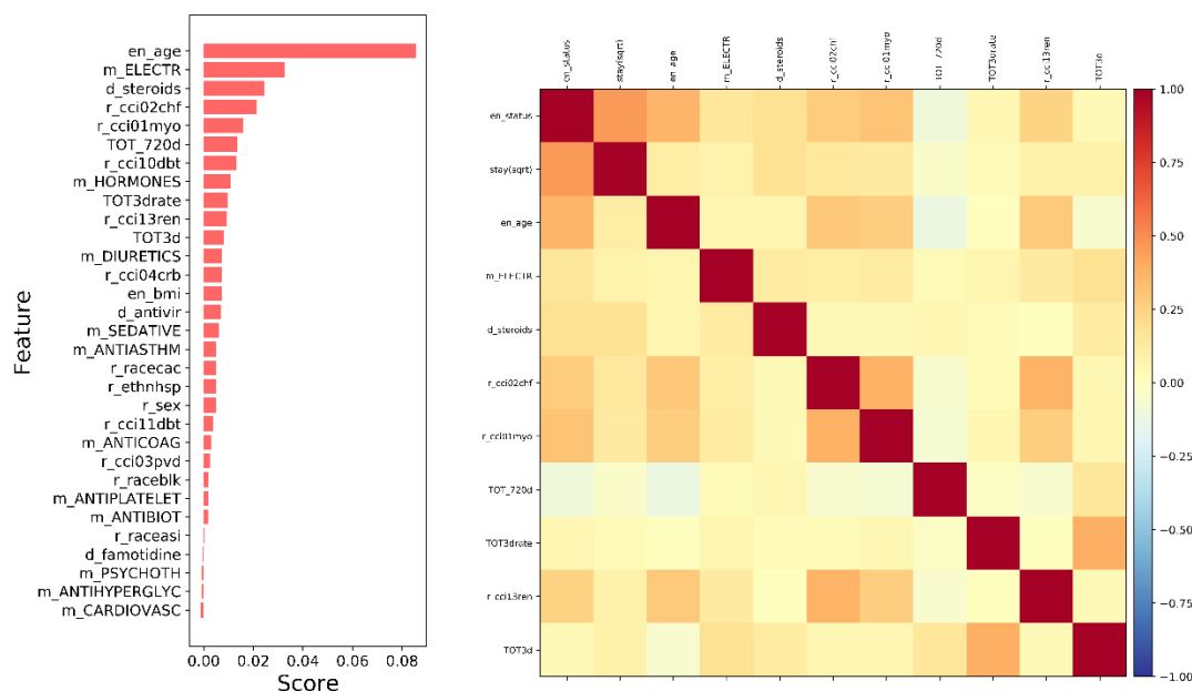
Figure 2. Features scoring for outcomes classification. (left) Permutation feature scoring. (right) Cross-correlation by using Pearson correlation coefficient R ranging from -1 to 1 (the color bar).
