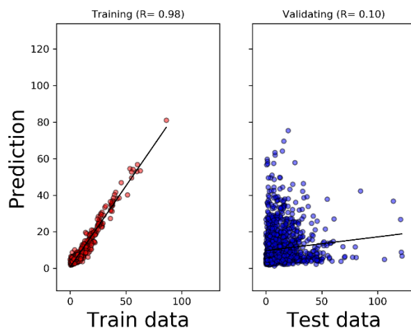
Figure 5. Regression model to predict hospitalization stay indicated further steps needed to optimize the model.
