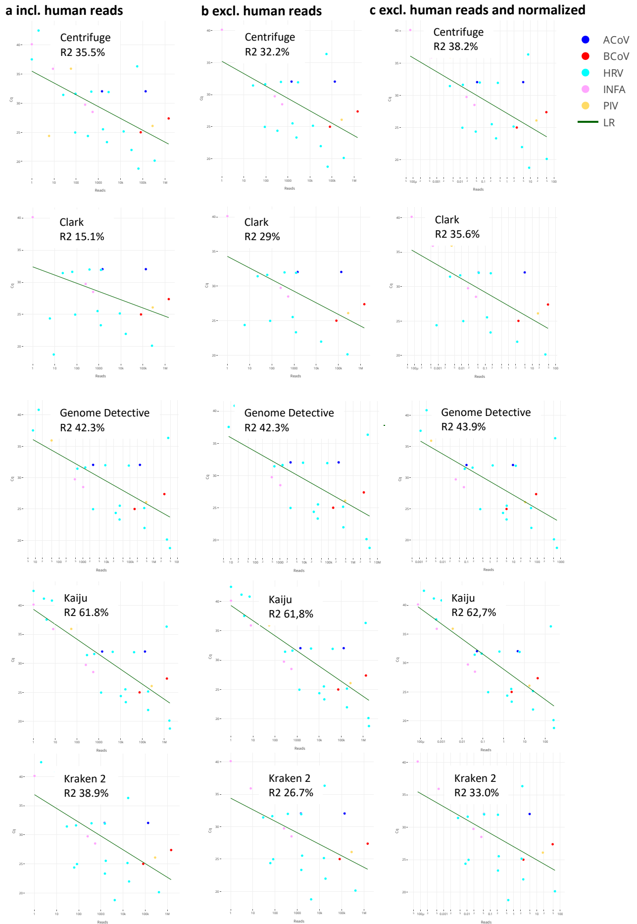
488 Figure 3. Correlation between the number of sequence reads assigned (species level) and Ct-values 489 of virus-specific PCRs, for the five taxonomic classifiers evaluated, a. without extraction of human 490 reads and b. after extraction of human reads, c. after normalization of reads by corresponding 491 genome lengths. 492
