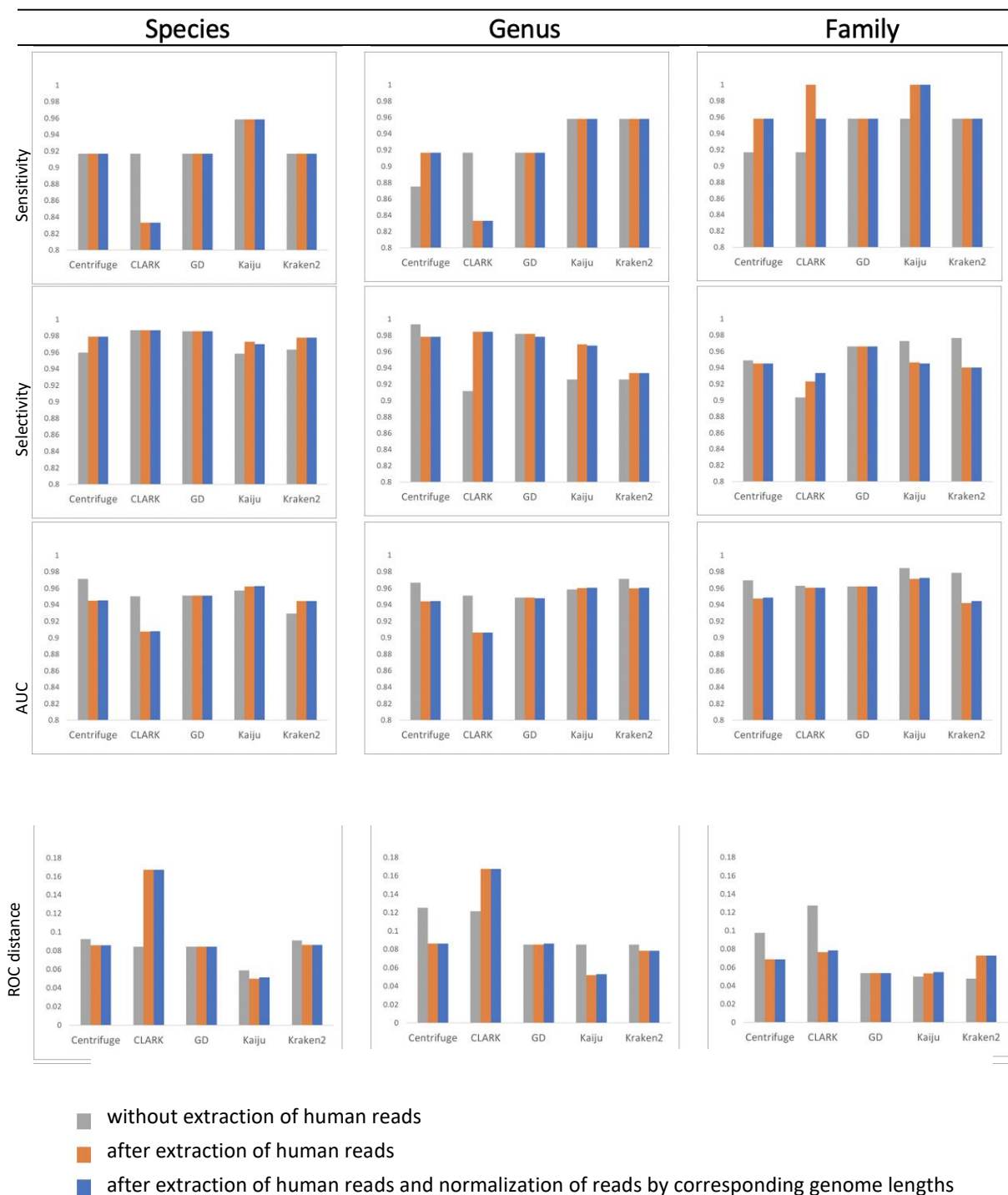
482 Figure 2. Sensitivity, selectivity, AUC, and ROC distance calculated based on assignment at three 483 taxonomic levels (species, genus, and family) by the five classifiers for three type of pre-processing 484 of the NGS datasets, a. without extraction of human reads and b. after extraction of human reads, c. 485 after extraction of human reads and normalization of reads by corresponding genome lengths. 486 487
