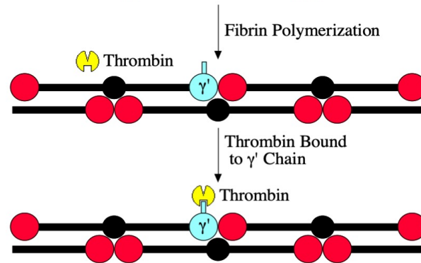
Fig 4. Model of \gamma' Fbg mechanism of thrombosis.
