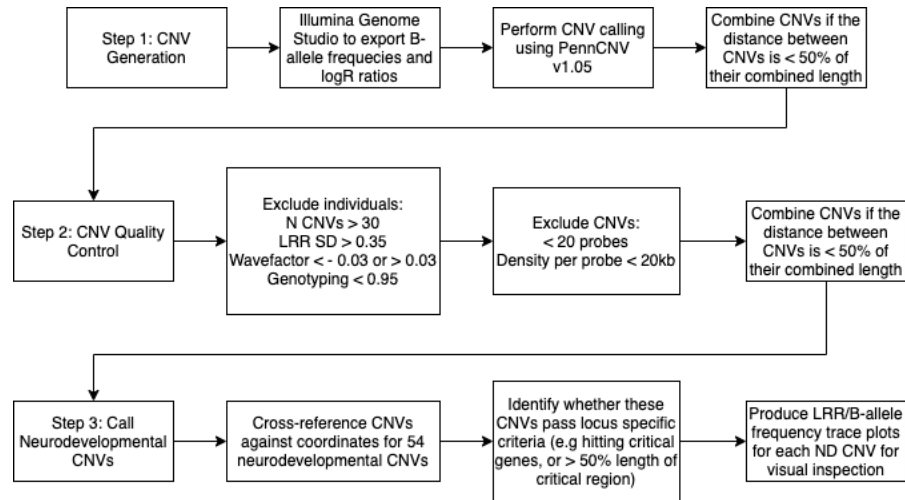
Figure 3 - DRAGON-Data pipeline for CNV Calling
