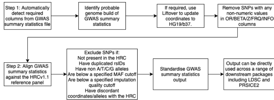
Figure 4 - DRAGON-Data Pipeline for standardising genome-wide association summary statistics (summaRygwasqc)
