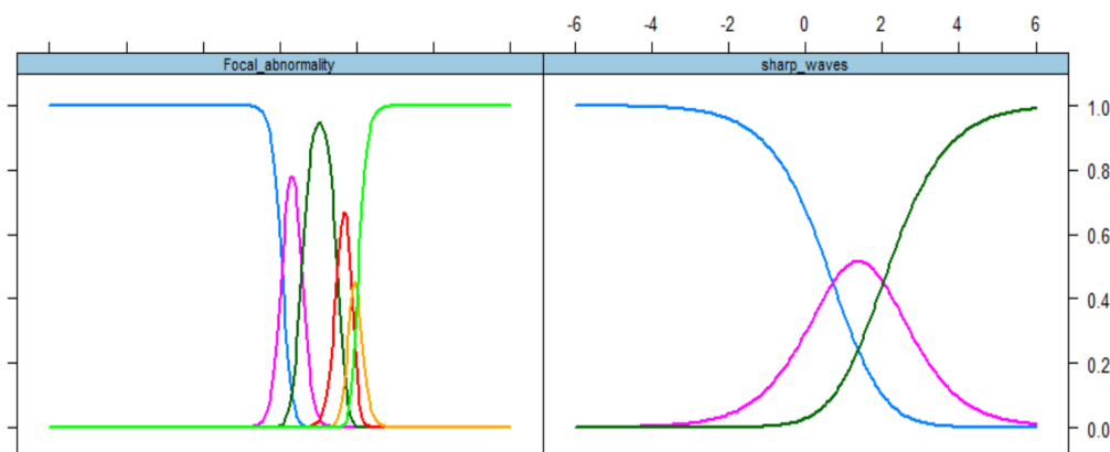
Figure 1. Trace/ICC plots. The x-axis is the value of the latent variable ( \theta ), and the y-axis is the probability P(\theta) that shows the chance of occurrence for each response category across different levels of \theta . Top Left: Focal Abnormality, the item with the best discrimination (0.97) Top Right: Sharp wave the item with worst discrimination (0.53).
