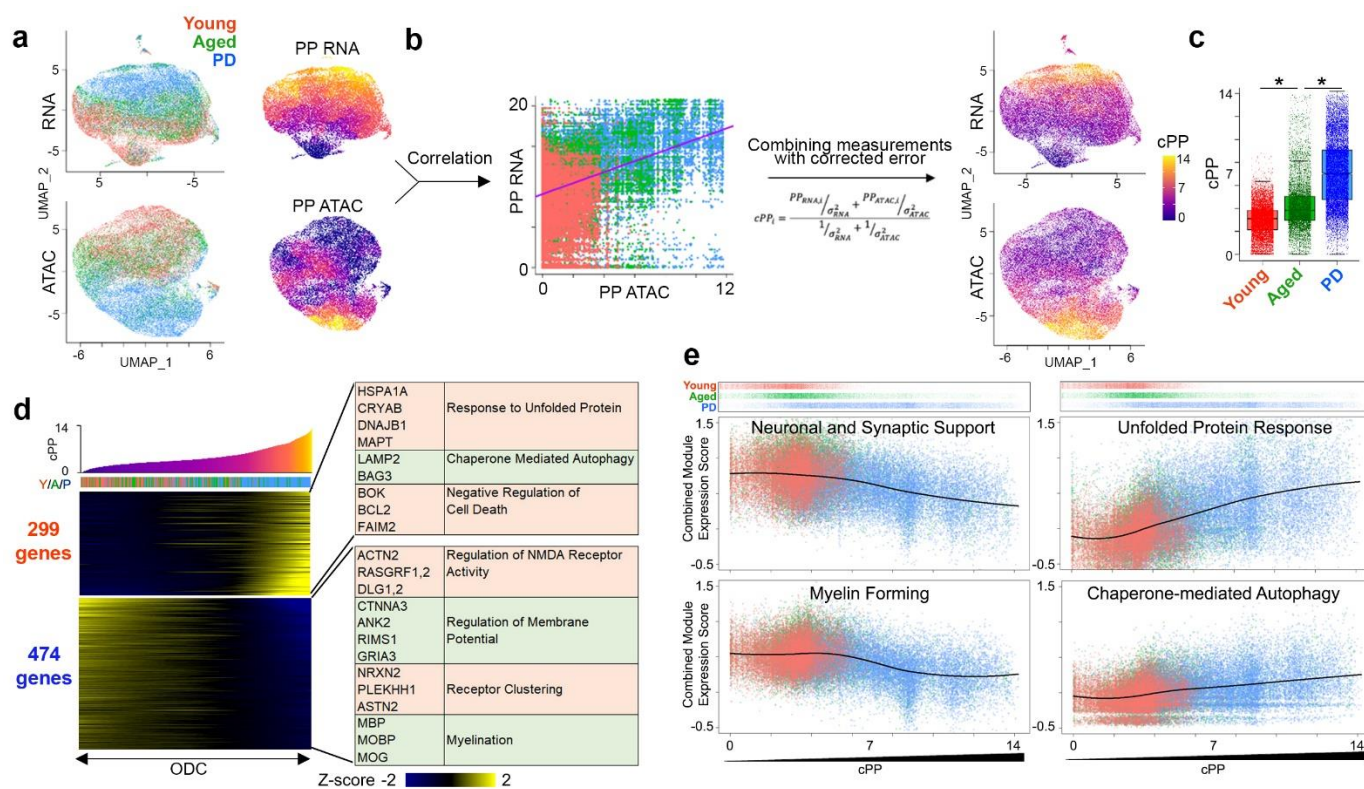
Fig. 3 | Establishment of pseudopathogenesis trajectory in ODC. a , UMAP plot of ODC nuclei colored by young, aged and PD donor (left), and heatmap of RNA- and ATAC-based pseudopathogenesis trajectory (right). b , Schematic of calculation of combined pseudopathogenesis (cPP) score from transcriptome and ATAC profiles. Cor = -0.419 ( p < 2.2e-16 ). c , Significant difference in cPP scores of individual ODC nuclei from young, aged and PD midbrain. (One-way ANOVA, p -value for Y/A < 1e-199 , p -value for A/P < 1e-199 ). d , Heatmap showing genes correlated with cPP trajectory. X-axis represents individual cells sorted by cPPs. Y-axis of heatmap represents positively (upper)- and negatively (bottom)-correlated genes. Representative genes and significant GO terms are shown in right panel ( Cor > 0.1 or < -0.1 ). e , Change in gene expression modules across cPP trajectory in ODC. Top panel shows individual ODC nuclei along cPP scores and donor group. X-axis shows cPP score. Y-axis is combined expression score for all genes in the expression module.
