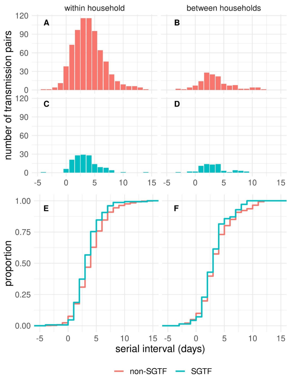
Figure 1. Observed distribution of serial interval of SARS-CoV-2 transmission pairs with infectors having their symptom onset date during the period 13 - 19 December 2021 in The Netherlands, (A) for non-SGTF within-household transmission pairs, (B) non-SGTF between-household transmission pairs, (C) SGTF within-household transmission pairs, (D) SGTF between-household transmission pairs, and the difference between the empirical cumulative density functions for SGTF and non-SGTF transmission pairs (E) within households and (F) between households (see Appendix for data).
