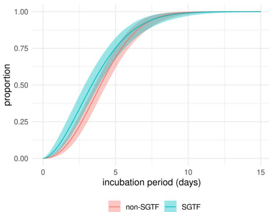
Figure S1 Estimated cumulative density function of the incubation period for 163 non-SGTF cases and 117 SGTF cases, with a symptom onset date between 1 and 26 December 2021.
