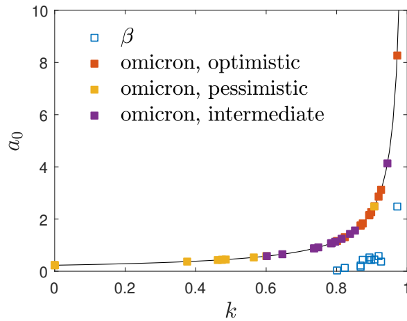
FIG. 2. Location of the considered values of a_0 and k for the omicron mutant in the investigated 12 countries with the adopted 3-day early doubling times. The symbols \beta represent the values for the earlier beta mutant. The solid black line is Eq. (23).
