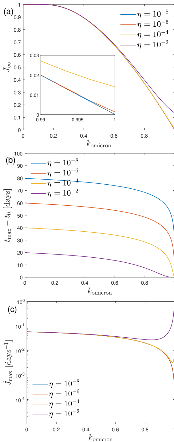
FIG. 1. (a) J_\infty , (b) t_{\max} - t_0 , and (c) j_{\max} as a function of the only parameter k for different values of the initial fraction of infected persons \eta in the case of an early 3-day doubling time.
