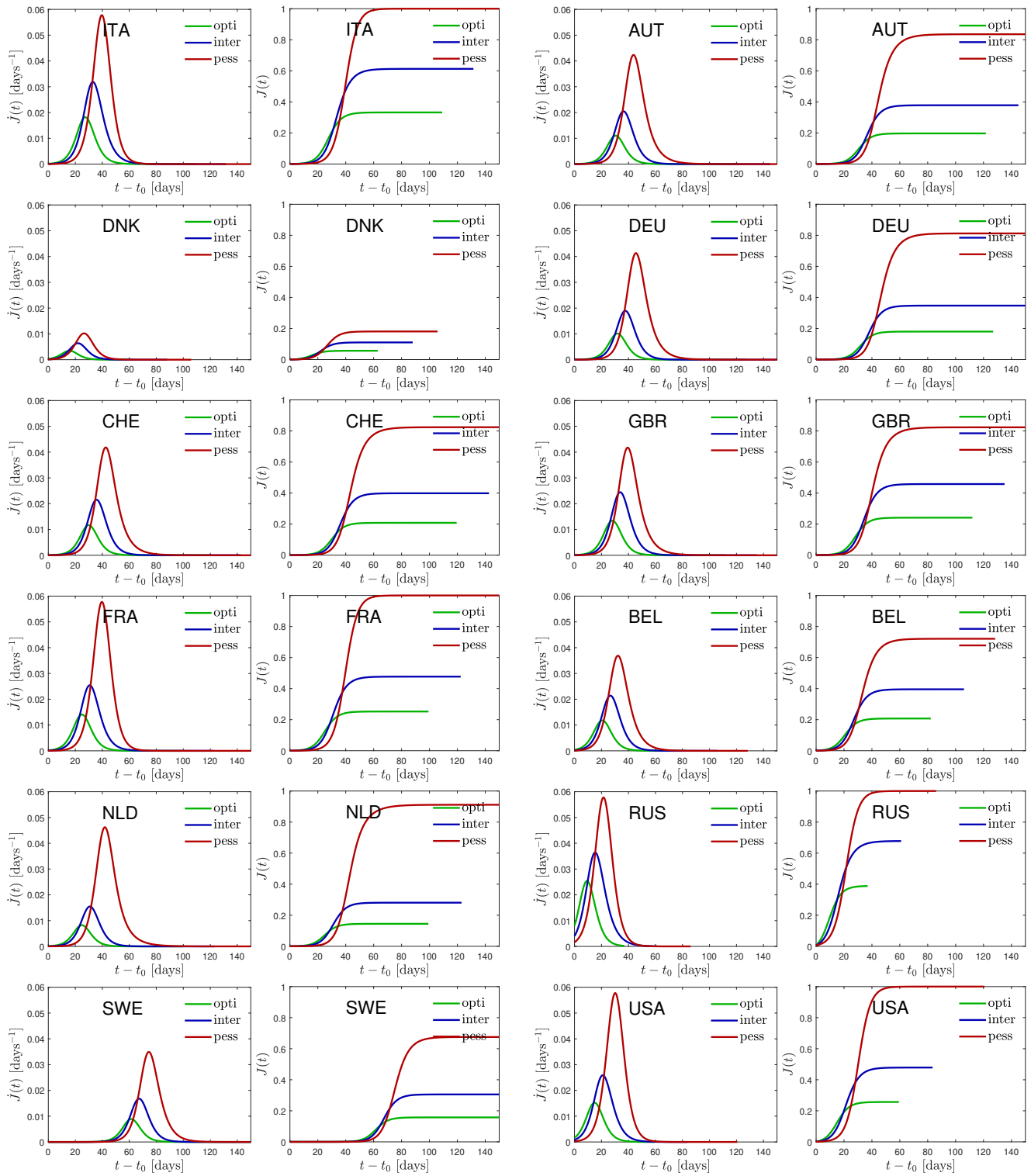
FIG. 3. Time dependence of the daily rate of newly infected persons, \dot{J}(t) , as well as the cumulative fraction of infected persons, J(t) , for all 12 countries.
