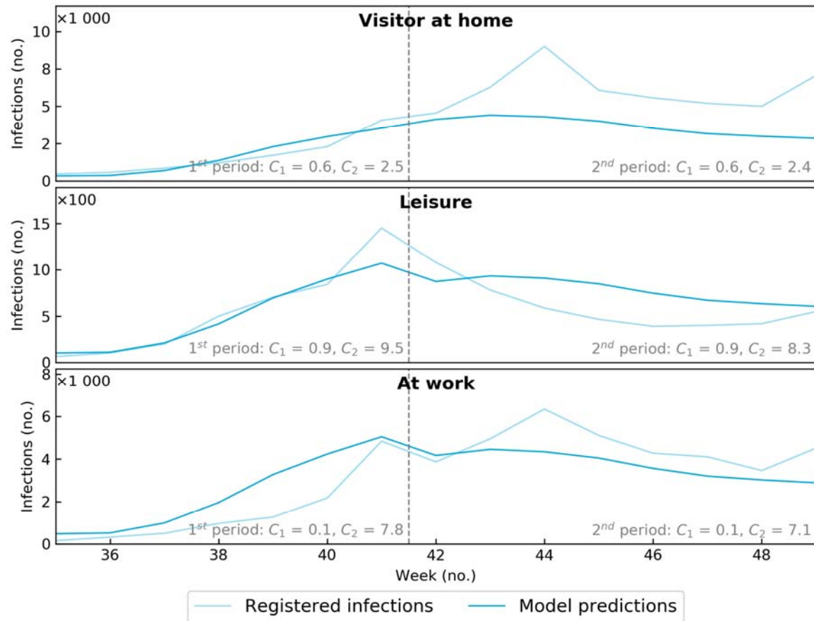
Figure 1: Number of infections based on internal validation by reproduction of infections at work, visitor at home and leisure.
