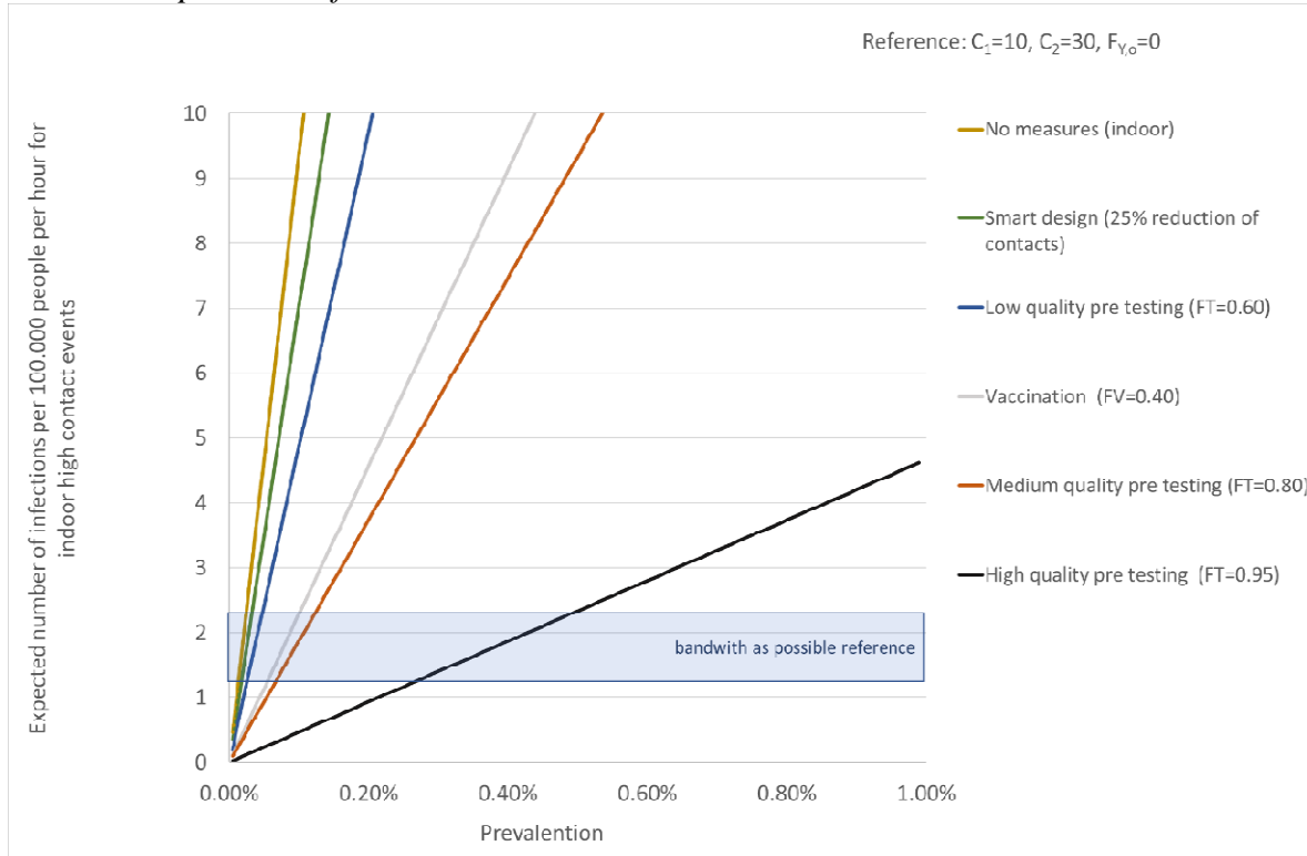
Figure 2: Risk of infections as a function of the prevalence for different packages of measures, related to a possible reference.
