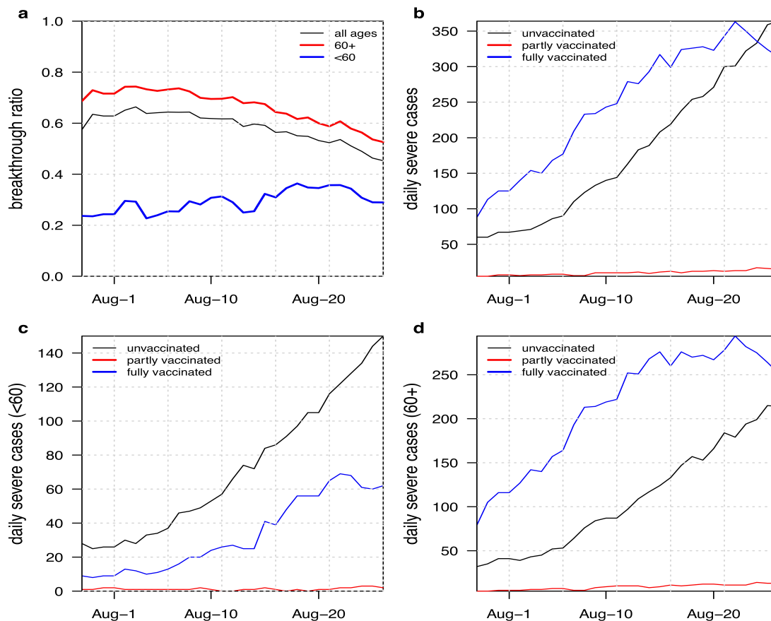
Figure 6. (a) Breakthrough infection ratio among severe cases ( BTI\_Ratio_i\_severe ) over time for all ages, age 60+ and age <60. (b) Daily reported severe cases for three types (unvaccinated, partly vaccinated, fully vaccinated) for all ages over time. (c) three types of daily severe cases for <60 years old. (d) three types of daily severe cases for 60+ years olds.
