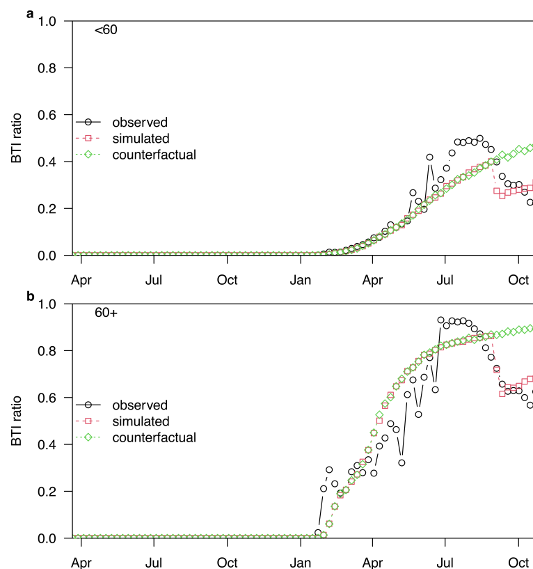
Figure 5. The observed (black circles) versus the simulated BTI ratios under factual (red squares) and counterfactual (green diamonds) scenarios for <60 age group (a) and for 60+ age group (b). These results correspond to Figure 4, showing the BTI ratio instead of case numbers.
