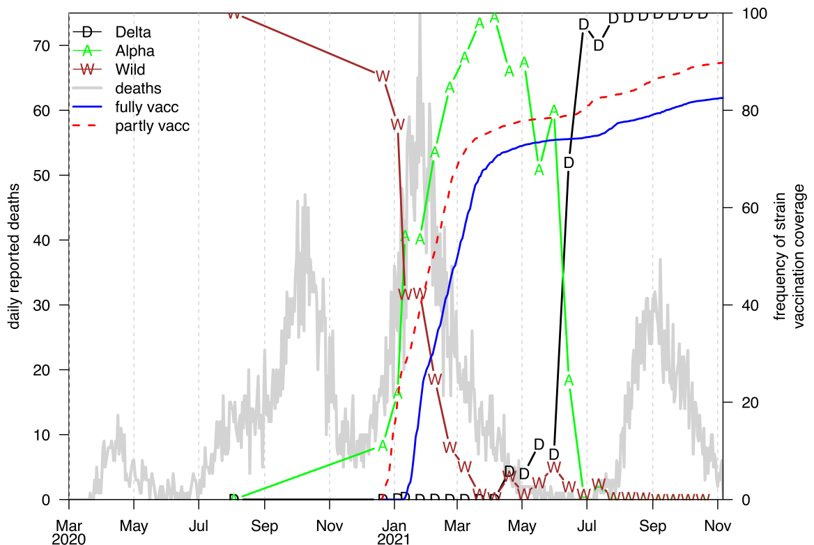
Figure 1. Daily reported COVID-19 deaths (grey) over pandemic period. Colored symbols show frequency of individual strains (as a percentage) of all strains sequenced (mostly biweekly) in Israel. Also plotted is the vaccination coverage (ie. proportion of the population being vaccinated) with solid blue representing fully vaccinated and red dashes for partially vaccinated (one dose). The Alpha variant replaced the wild-strain in December 2020-February 2021, while the Delta replaced the Alpha variant in June-July 2021. The final wave in the graph is almost completely due to the Delta variant.
