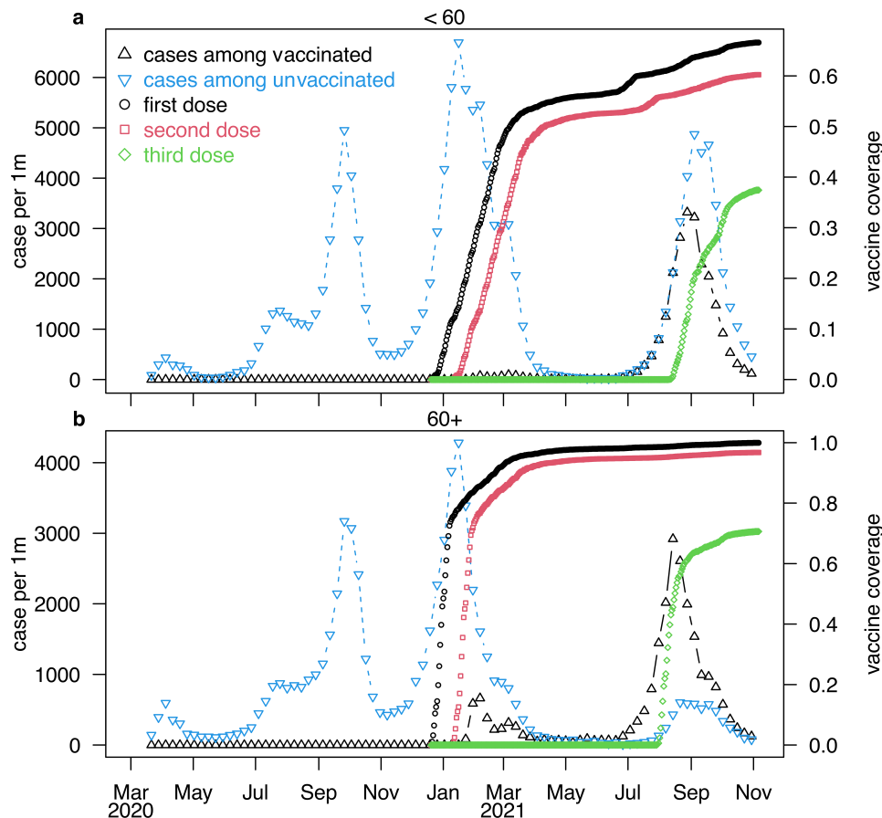
Figure 3. Infection and vaccination dynamics in Israel. Weekly reported COVID-19 cases are presented for the <60 (a) and 60+ (b) age groups (population standardized, per 1 million individuals in an age group), in unvaccinated (blue, down-facing triangles) and fully vaccinated (black, up-facing triangles) individuals. The cumulative vaccine coverage for the first, second and third dose are represented by black circles, red squares, and green diamonds, respectively.
