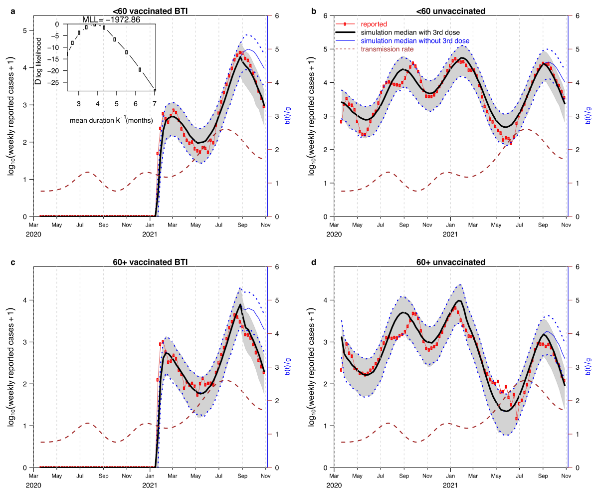
Figure 4. Model fitting results. The mean simulated cases (black bold) versus observed cases (red circles) for the <60 age vaccinated group in (a); for the <60 unvaccinated group in (b); for the 60+ vaccinated group in (c) and for the 60+ unvaccinated group in (d). Note that a logarithmic scale is used. The cases in (a,c) are BTIs. The brown dashed curve shows the transmission rate. The inset in panel (a) shows the profile maximum log-likelihood as a function of \kappa , and used to determine the best estimate of \kappa . The blue thin curves show the counterfactual scenario where the effect of the third dose is shut off by fixing \varepsilon = 0.8 constant. The two dotted blue curves show the 95% range of the 1000 simulations when the effect of third dose is shut off and it is possible to see infective numbers in this scenario (Scenario 2).
