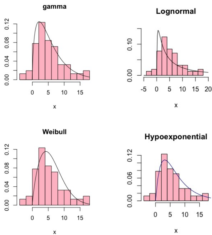
Figure 12: Fitted distributions with the method of moments
