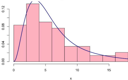
Mixture of gamma SI distribution
