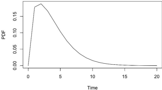
Generation Time distribution
