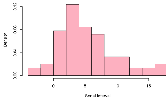
Figure 11: Histogram of the serial interval
