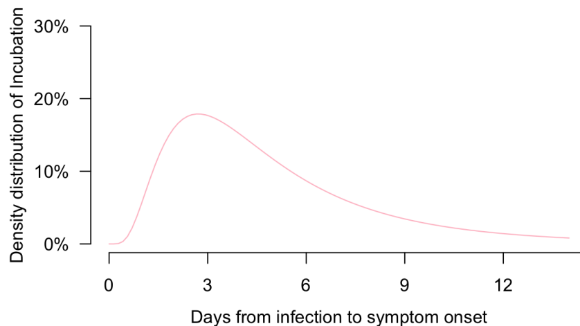
Figure 19: Density distribution of incubation by a best-fit log-normal distribution with parameters 1.4340 and 0.6612
