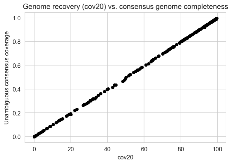
S. fig. 2. Genome recovery vs. unambiguous consensus genome coverage. Pearson R > 0.99999 , p < 0.00001 .
