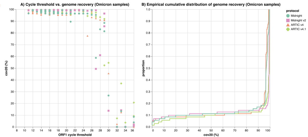
Fig. 4. A) Comparison of existing and revised (v2) Midnight protocols in terms of ORF1 cycle threshold vs. genome recovery (cov20) in sample set 4, which comprises Omicron lineage samples selected by S gene target failure. LOESS lines omitted here for lack of data. B) Cumulative empirical cov20 distributions for existing and revised Midnight protocols.
