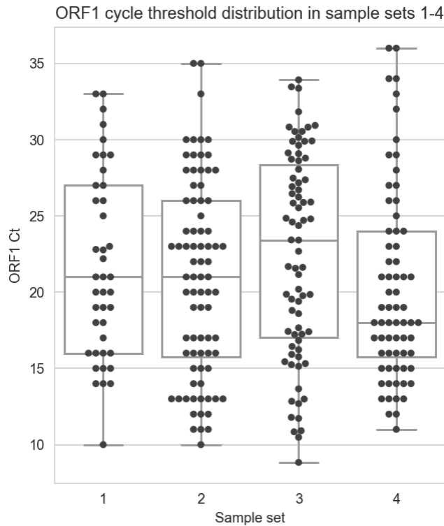
S. fig. 1. TaqPath RT-PCR ORF1ab cycle threshold distribution for sample sets 1-4.
