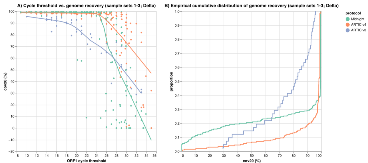
Fig. 2. A) TaqPath ORF1 gene cycle threshold (Ct) vs. genome recovery at \geq depth 20 (cov20) in 196 Delta lineage samples with LOESS regression lines. B) Empirical cumulative distribution of cov20. ARTIC v4 yielded much higher typical genome recovery than Midnight in low viral titre, high Ct samples while Midnight recovered more genome in high viral titre, low Ct samples. Shown are sample sets 1-3 for Midnight and ARTIC v4, and sample set 1 only for ARTIC v3, which performed poorly.
