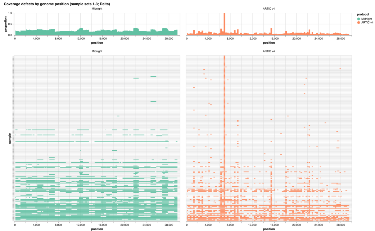
Fig. 3. Coverage defect distribution (depth < 20) in 196 Delta lineage SARS-CoV-2 clinical samples, sorted by ascending ORF1 gene Ct value. ARTIC v4 exhibited a systematic defect at approximately 6850-7080bp (S gene) (right).
