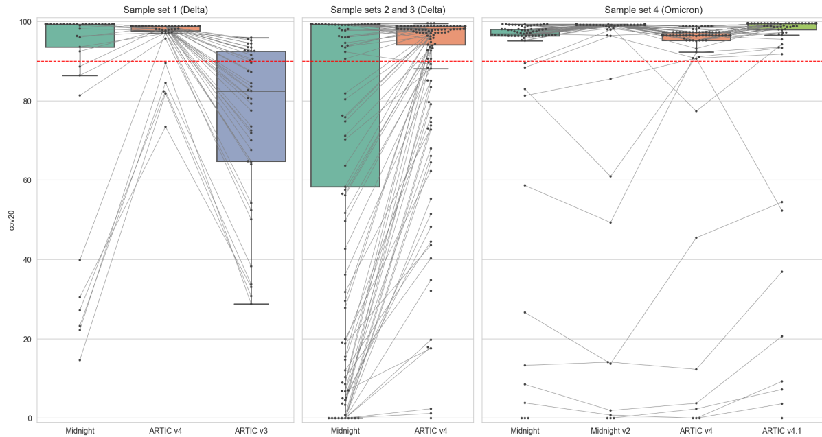
Fig. 1. Genome recovery at or above depth 20 in head-to-head sequencing of 196 Delta and Omicron lineage SARS-CoV-2 clinical samples over a total of 9 runs. Red lines correspond to a widely used lower bound on genome recovery for lineage assignment (90%).
