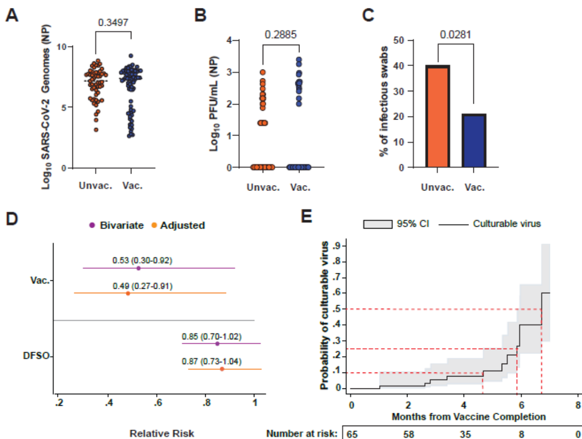
Figure 1. Isolation of infectious SARS-CoV-2 from vaccinated and unvaccinated individuals reveals waning protection beginning at 5 months. (A) Violin plots of \text{log}_{10} transformed SARS-CoV-2 viral genomes from nasopharyngeal swabs from vaccinated and unvaccinated individuals. Copy number estimates of SARS-CoV-2 viral genomes were performed using linear regressions to correct for differences in clinical testing platforms and nucleic acid isolation procedures (Extended Methods). Solid lines represent the median values, and dashed lines represent quartiles within each group. Significance was assessed using a two-tailed, unpaired Student's t-test with Welch's correction for unequal variances ( t=0.9388 , df=122.8 ). Exact p-values are reported. (B) Violin plots of \text{log}_{10} transformed particle forming units / mL (PFU / mL) of infectious virus isolated from nasopharyngeal swabs from vaccinated and unvaccinated individuals. Solid lines represent the median values, and dashed lines represent quartiles within each group. Significance was assessed using a two-tailed, unpaired Student's t-test ( t=1.066 , df=123 ). Exact p-values are reported. (C) Proportion of swabs with infectious virus for unvaccinated and vaccinated individuals. Significance was assessed using Fisher's Exact test and P-value threshold is reported. (D) Relative risk of isolating culturable virus amongst vaccinated and unvaccinated individuals with COVID-19 infection and the 95% confidence intervals in parenthesis. Significance was assessed using robust standard errors (E) Probability of culturable virus from time to completion of vaccination (black) along with respective 95% confidence intervals (grey) amongst those with completed mRNA vaccination schedules. Red dashed lines indicate fixed levels of probability of culturing infectious virus (10%, 25%, and 50%) with corresponding months since vaccine completion. Abbreviations (left to right): NP = nasopharyngeal; Unvac. = Unvaccinated; Vac. = Vaccinated; PFU = plaque forming units; DFSO = Days from symptom onset; CI = Confidence Interval.
