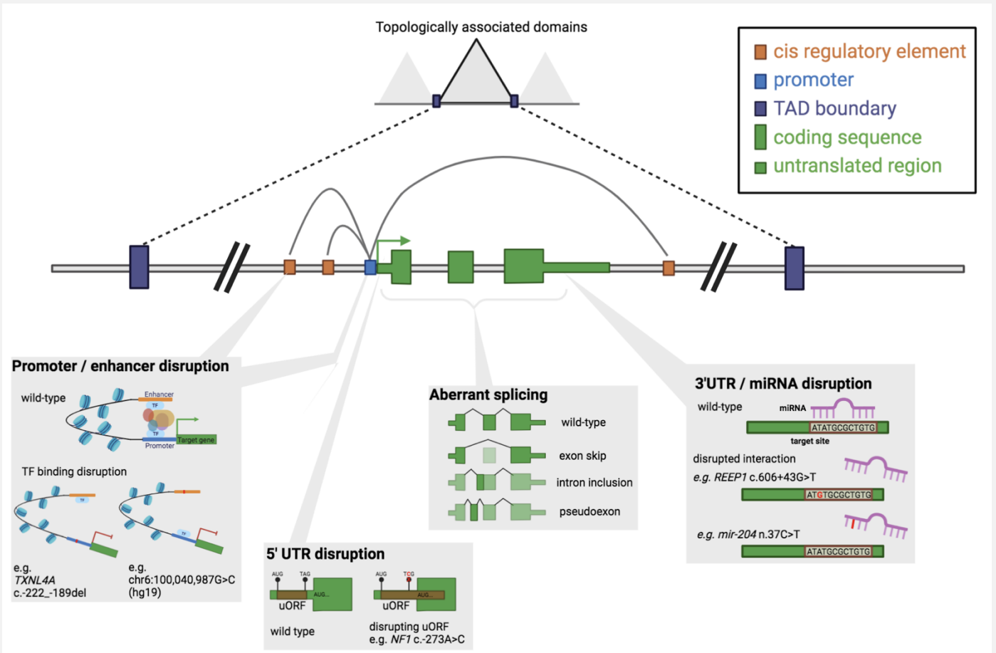
Figure 1: Schematic of regulatory elements within and around a gene and examples of disruptions that can lead to disease.
