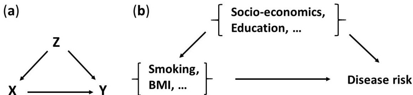
Figure 1: Consider the influence of one or more exposures X , on diseases Y , with confounding variables Z that satisfy the “backdoor criteria” [1, 7] (figure a). For example, X might include BMI, alcohol, and smoking, with confounders Z of socio-economic status and education (figure b).
