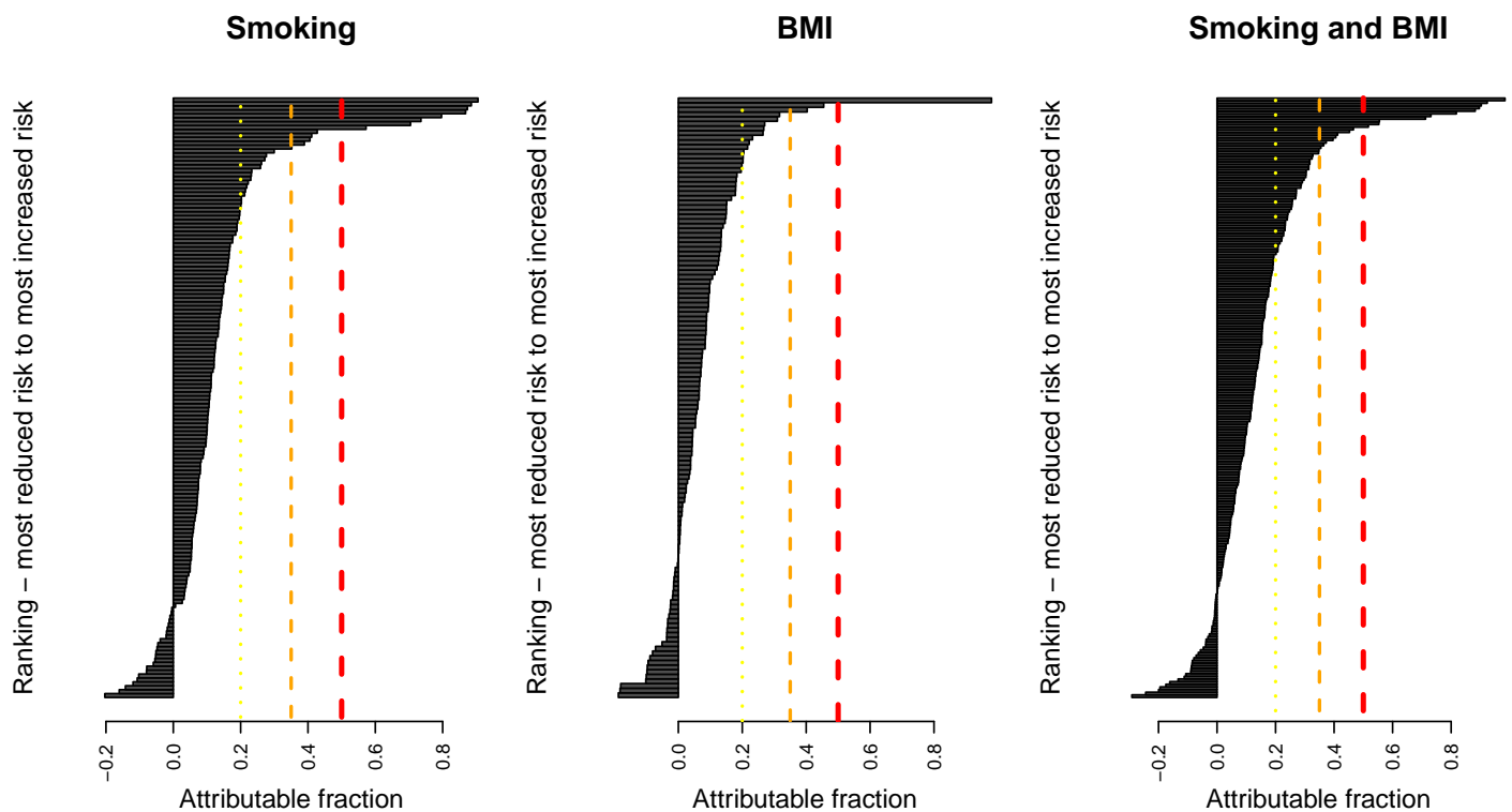
Figure 3: For diseases with a statistically significant association with smoking or BMI after an FDR multiple-testing adjustment, attributable fractions A_f were calculated with Eq. 10. Lines indicate A_f = 0.5 (red), A_f = 0.35 (orange), A_f = 0.2 (yellow). A_f < 0 indicates a protective association.
