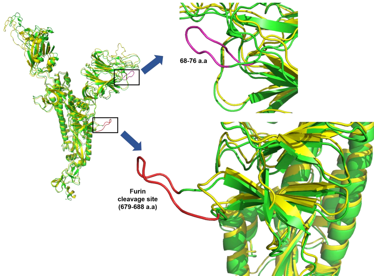
Figure 3: Superimposed structure of spike glycoprotein. The wild type spike glycoprotein is represented in green color while the structure of spike protein with deletions at site I and II is represented in yellow color. The 68-76 amino acid deletion in the N-terminal domain is shown in purple color (upper right panel) while 679-688 amino acids deletion is shown in red color (lower right panel).
