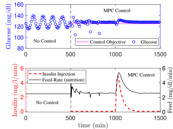
Fig. 4. Top panel: performance of the MPC control algorithm to maintain plasma glucose at a target level (control objective) against unknown insulin intervention to the real system (patient), applied at 1000 min; Bottom panel, feeding rate was adjusted by the controller to overcome the reduction in the plasma glucose by the insulin injection.
