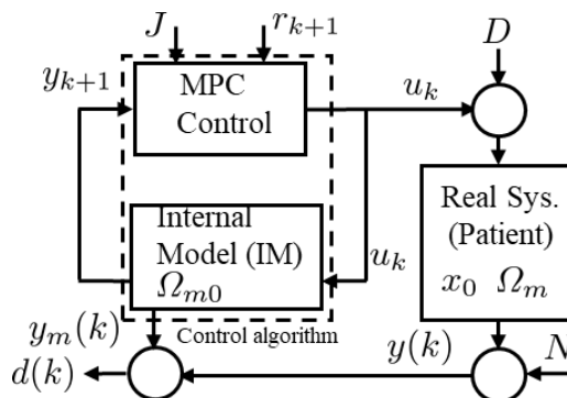
Fig. 2. Closed-loop MPC control algorithm with a state observer scheme (Kalman filter).
