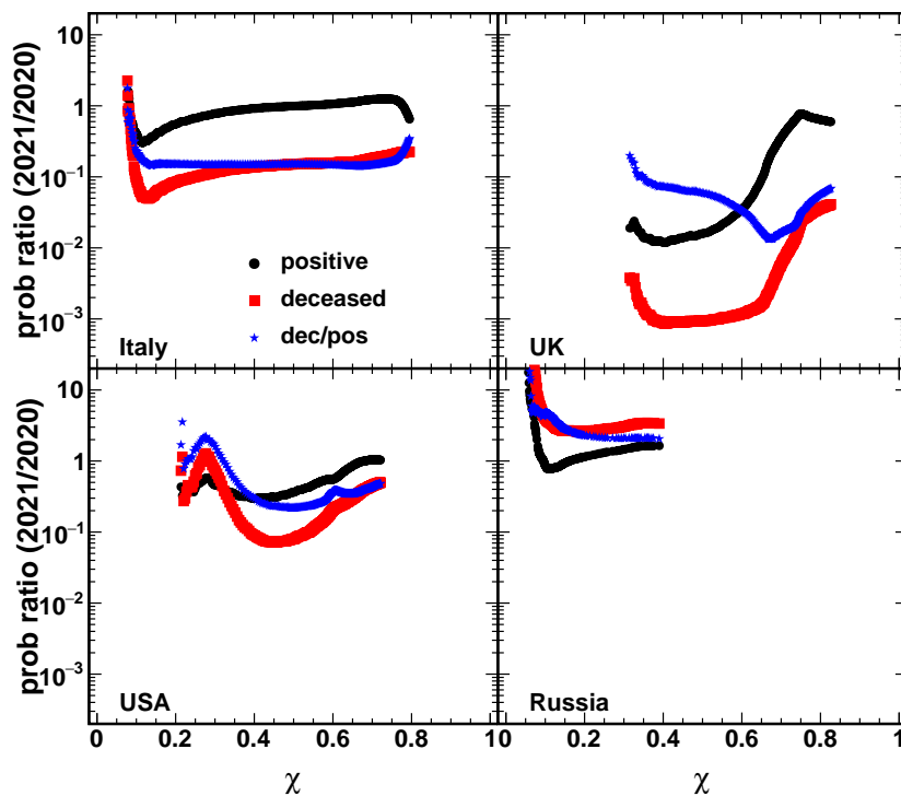
Fig. 4. (Color online) The probability ratio for the same period in 2021 and 2020 versus the vaccination ratio \chi for each country.
