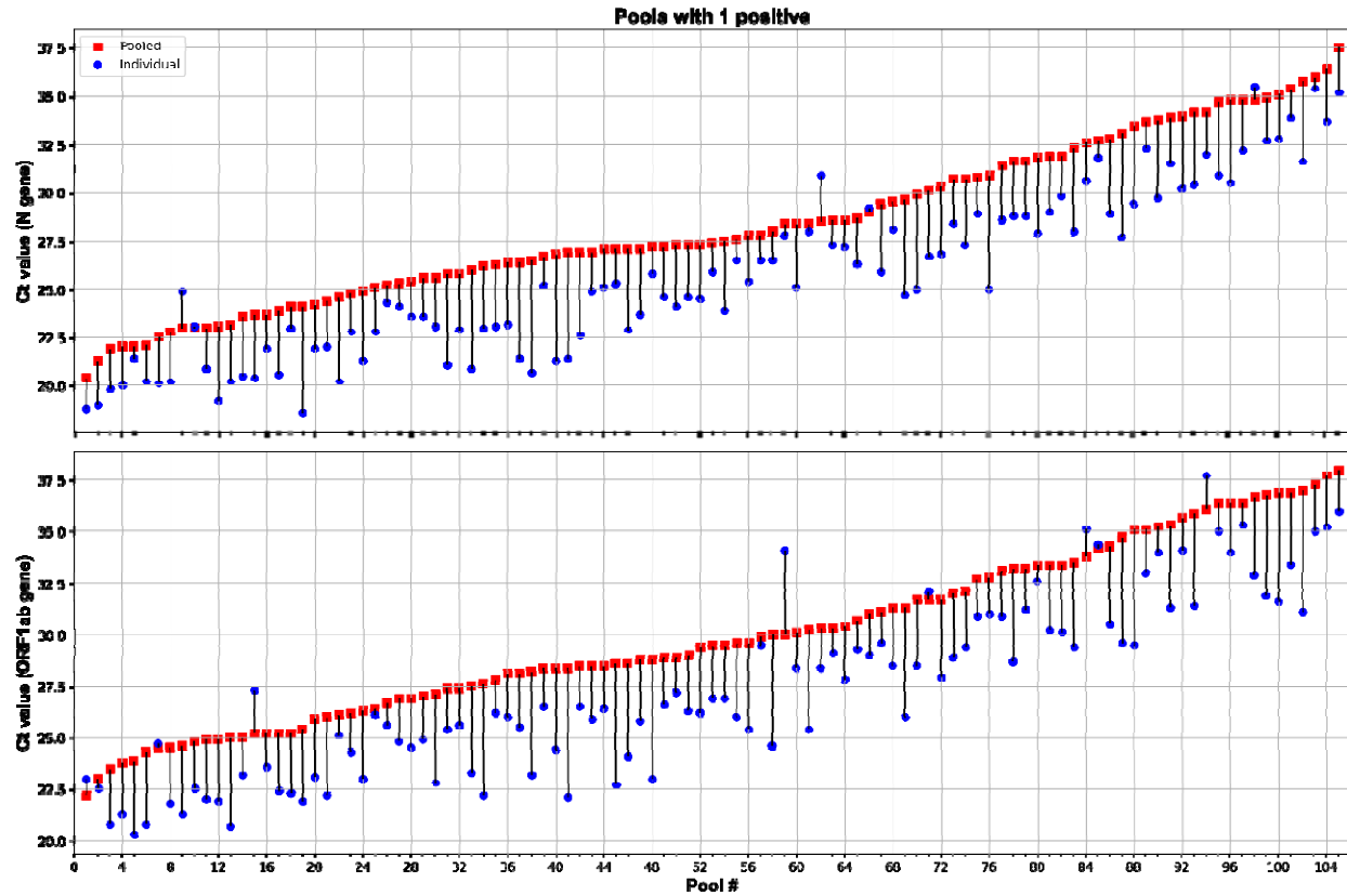
1 2 Figure 1. Pools with a single positive. Scatter plots showing cycle threshold (Ct) values and Ct shifts 3 detected by rRT-PCR in five-samples pools (squares), composed of four negative and one positive 4 samples, with respect to the individual positive samples (circles) for N (top graph) and ORF1ab (bottom 5 graph) genes. (2 column image)
