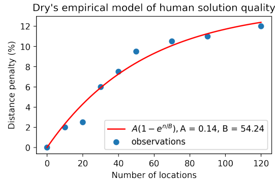
Figure 3: An empirical model of human performance on the TSP, taken from Dry's review [9]. The individual observations from that work are reproduced here; a curve fit of the form A(1 - e^{-n/B}) was performed to yield a smooth model. The penalty is less than 10% for problems sized up to around 60 locations.
