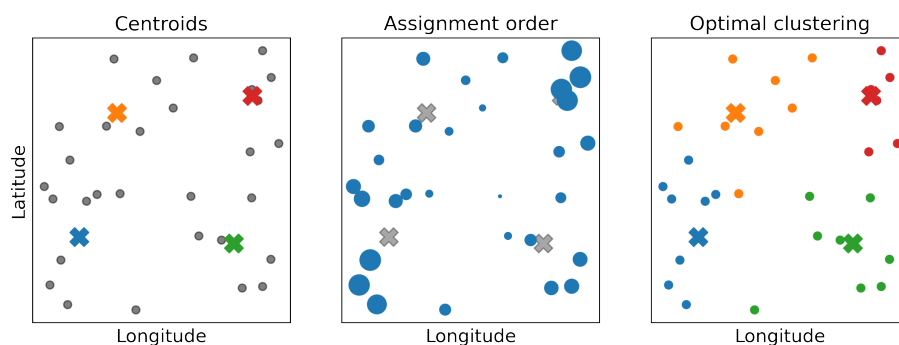
Figure 2: Example clustering of N = 30 patients into groups of D = 8 . Left: initialisation of four cluster centroids (denoted with crosses). Centre: order of patient assignment, where larger circles indicate priority. Patients in the centre of the distribution could be assigned to any cluster with low cost, so are dealt with last. Right: the optimal clustering of patients after assignment. The red cluster has six patients due to imperfect number division, whereas all other clusters are fully-sized.
