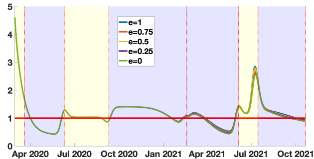
Figure 7: In this figure we plot the quasi-instantaneous reproduction number with vaccination R_V^0(t) = \frac{\tau(t)W(t)S_0}{\eta\nu} \times (\eta + \kappa\nu(1 - f)) . The blue background color regions correspond to epidemic phases, and the yellow background color regions to endemic phases.
