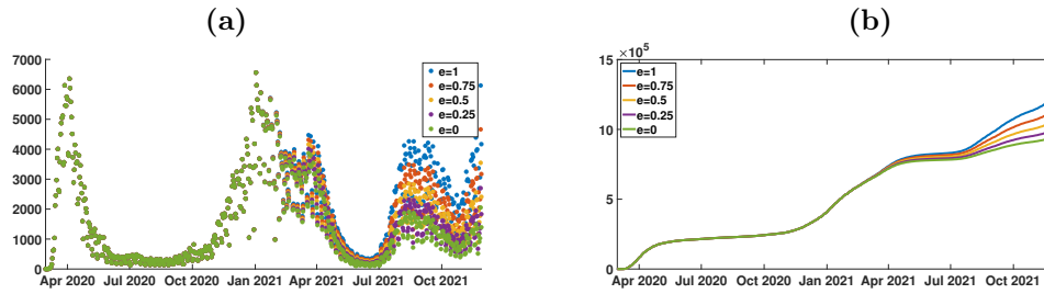
Figure 4: We plot \widehat{CR}_{\text{Data}}(t)' in (a), and we plot \widehat{CR}_{\text{Data}}(t) in (b) for New York City, and e = 0, 0.25, 0.5, 0.75, 1 . In (a), the green dots for e = 0 corresponds to the original daily number of reported cases CR_{\text{Data}}(t)' . In (b), the green curve for e = 0 also corresponds to the original cumulative number of reported cases CR_{\text{Data}}(t) .
