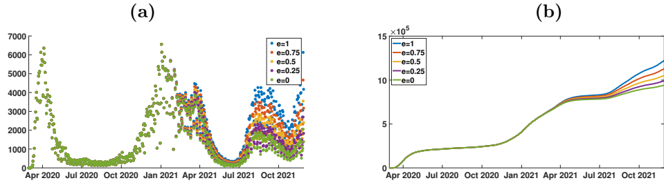
Figure 4: We plot \widehat{CR}_{Data}(t)' in (a), and we plot \widehat{CR}_{Data}(t) in (b) for New York City, and e = 0, 0.25, 0.5, 0.75, 1 . In (a), the green dots for e = 0 corresponds to the original daily number of reported cases CR_{Data}(t)' . In (b), the green curve for e = 0 also corresponds to the original cumulative number of reported cases CR_{Data}(t) .
